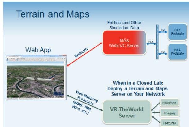
Figure 4. WebLVC Server integrated with VR-TheWorld Server
