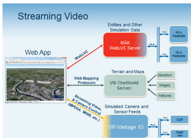
Figure 5. Streaming video
