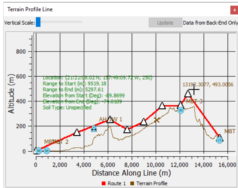
Figure 21. Terrain profile
