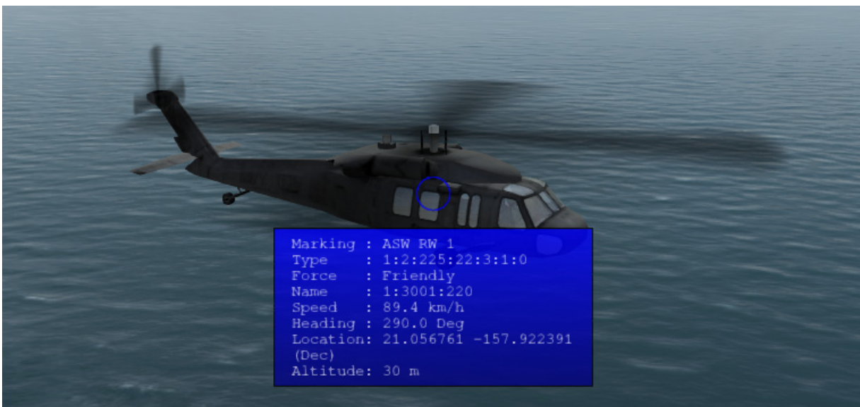
Figure 13. Entity label
