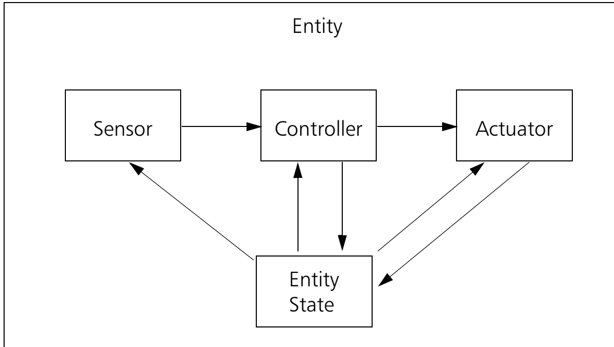
Figure 20. Entity component architecture
