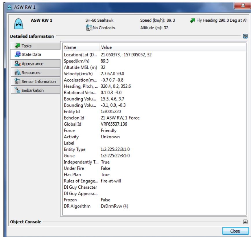
Figure 12. Information panel
