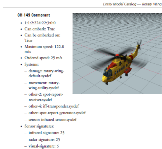
Figure 21. Model library
