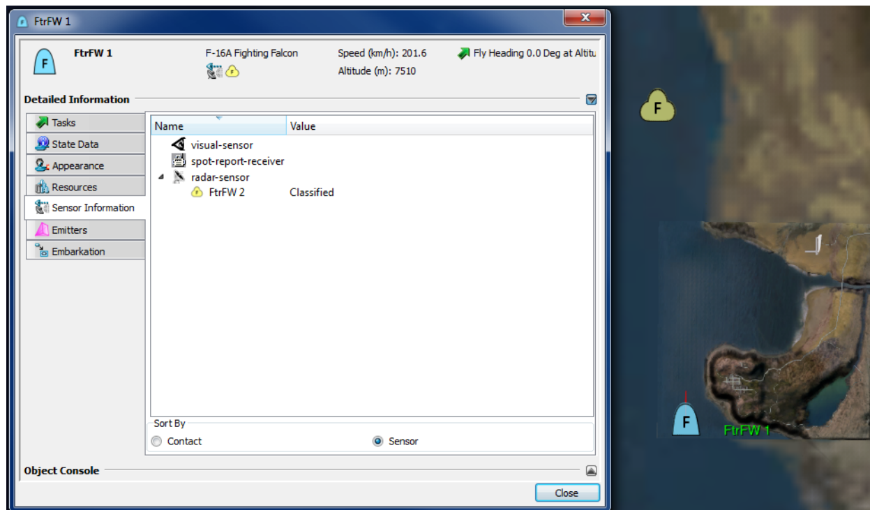
Figure 6. Combat identification
