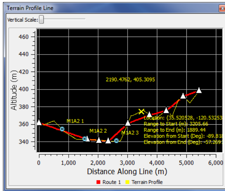
Figure 18. Terrain profile
