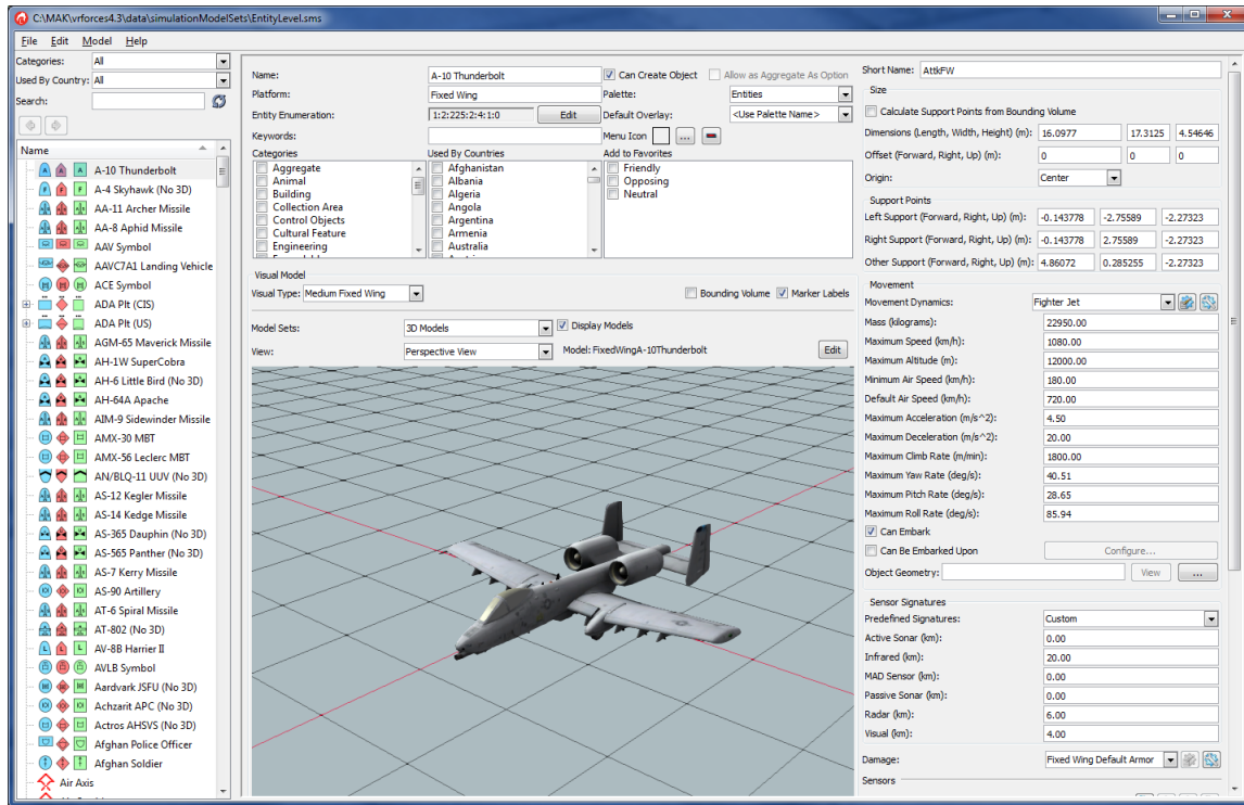
Figure 2. Entity Editor
