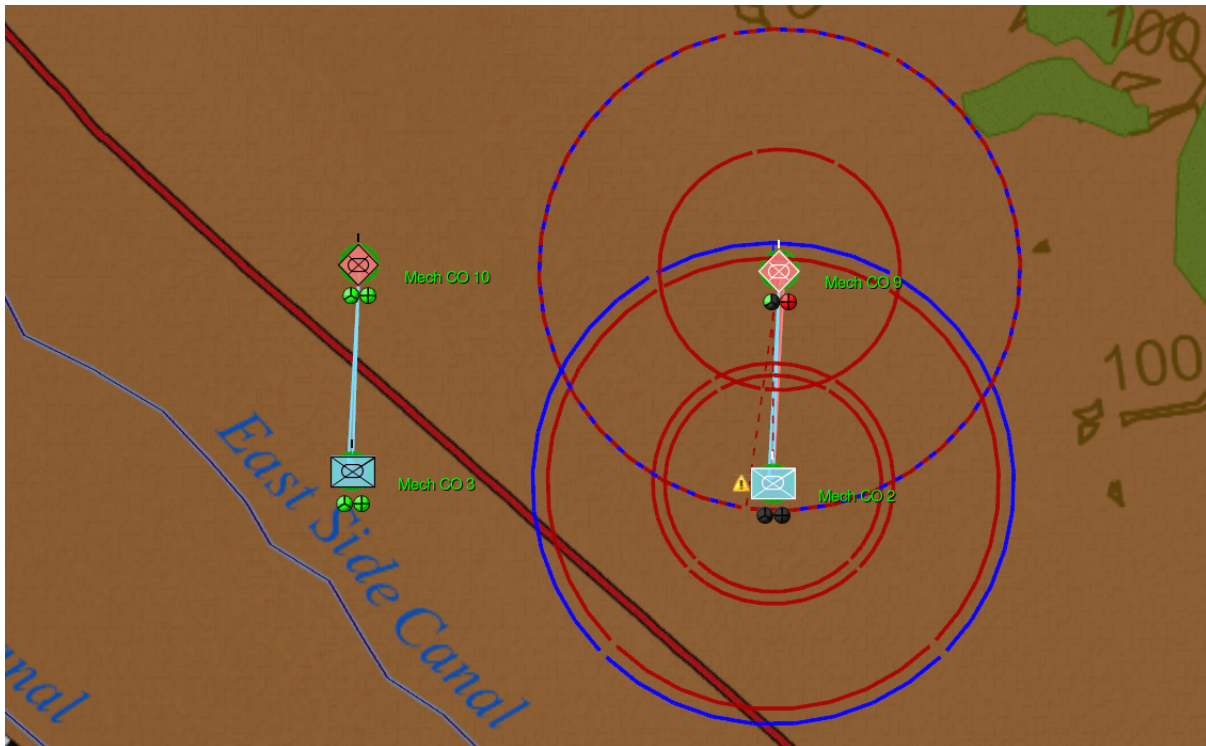
Figure 7. Aggregate combat
