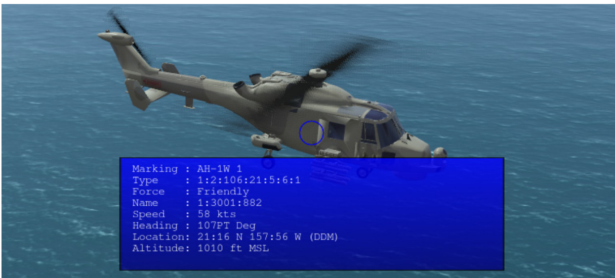
Figure 15. Entity label
