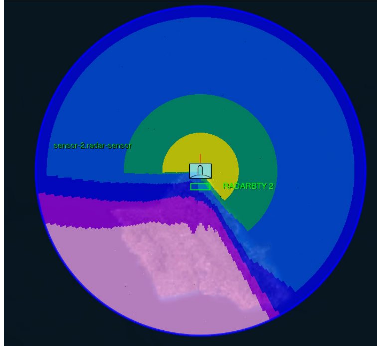
Figure 24. Radar Coverage
