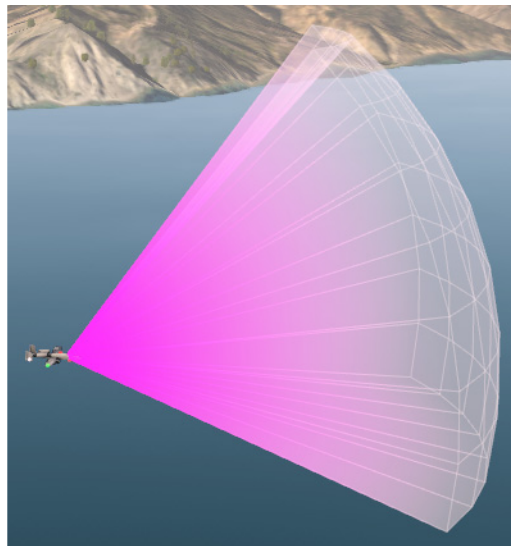
Figure 19. Electromagnetic emissions
