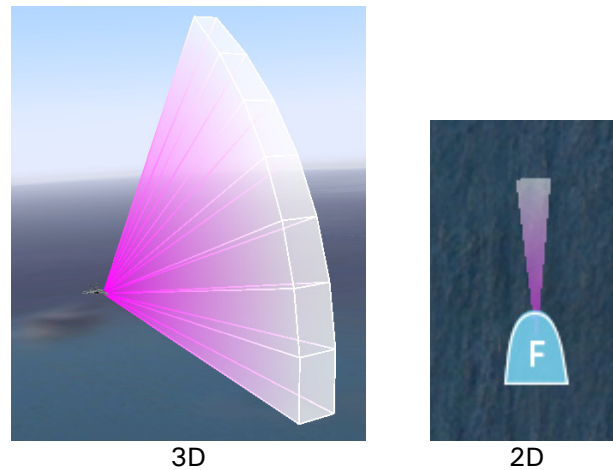
Figure 3. Emitter volumes
