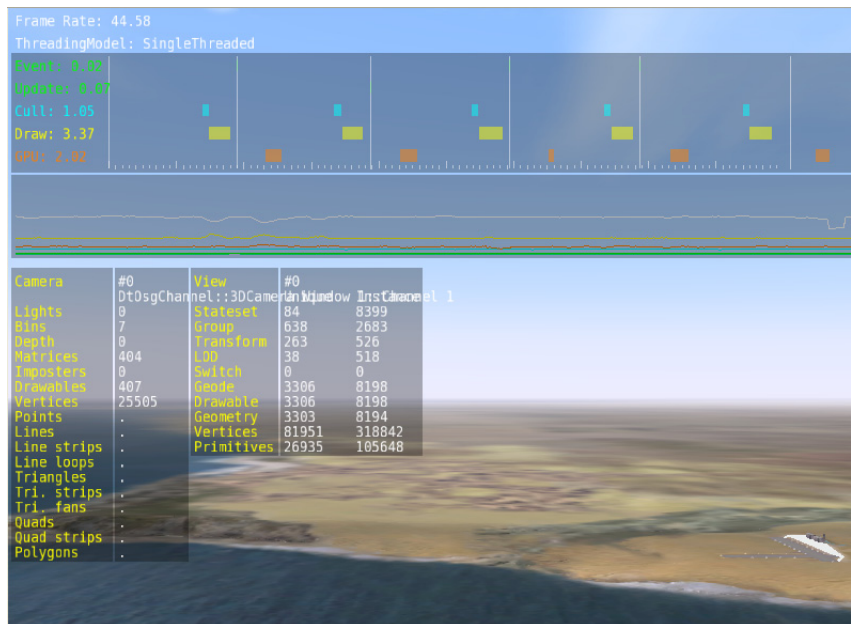
Figure 4. OSG performance statistics
