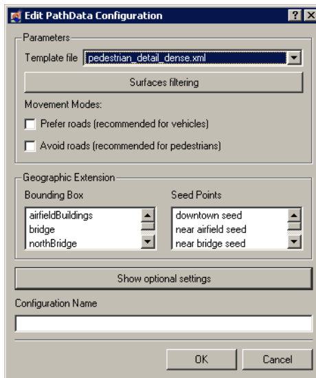
Figure 3-9. Edit PathData Configuration dialog box
