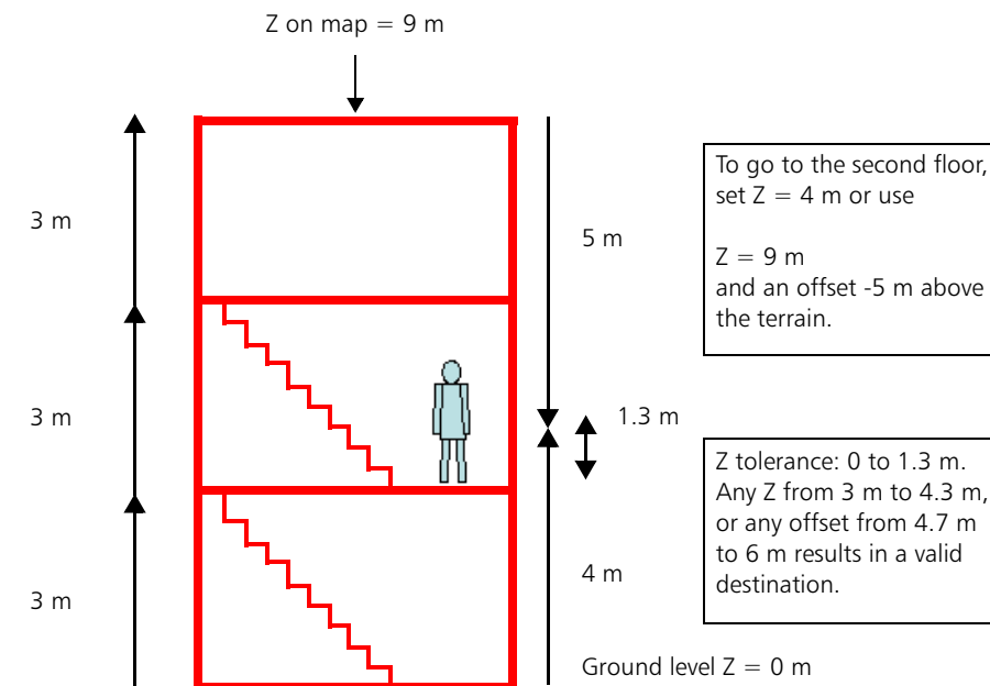
Figure 4-5. Specifying a location within a building
