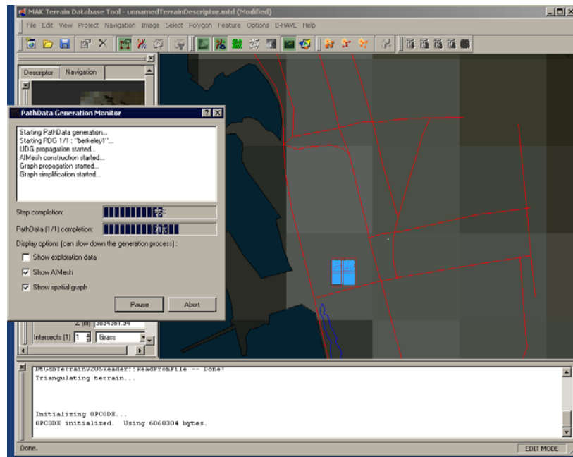
Figure 3-14. PathData generation
