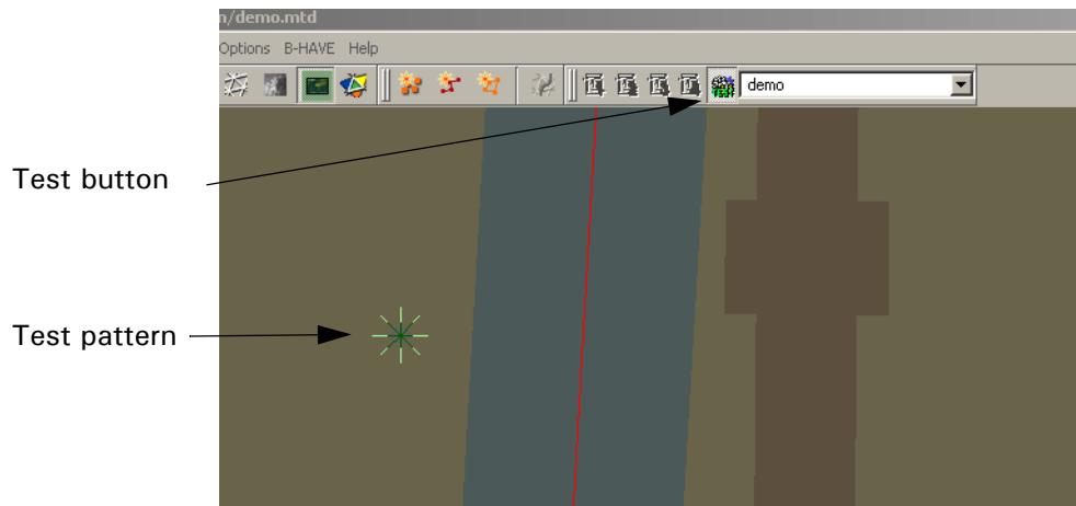
Figure 3-17. Testing PathData
