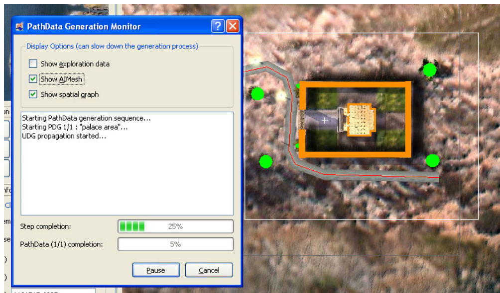
Figure 3-13. PathData generation
