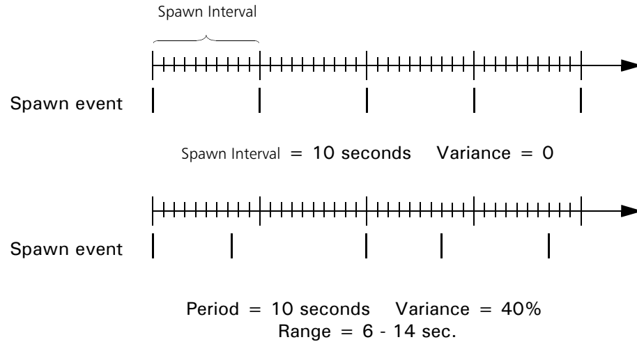
Figure 5-5. Spawn period and variance
