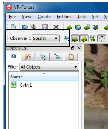
Figure 3. Observer mode
