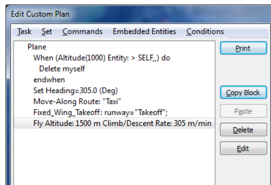
Figure 19. Custom plan
