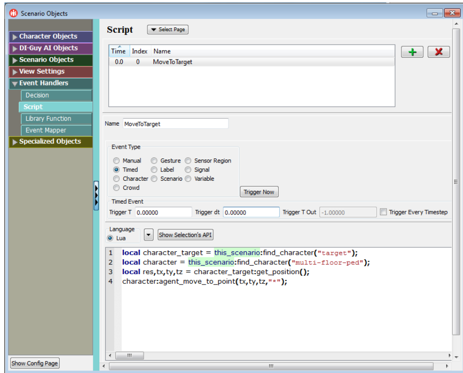
Figure 3-28. MoveToTarget script
