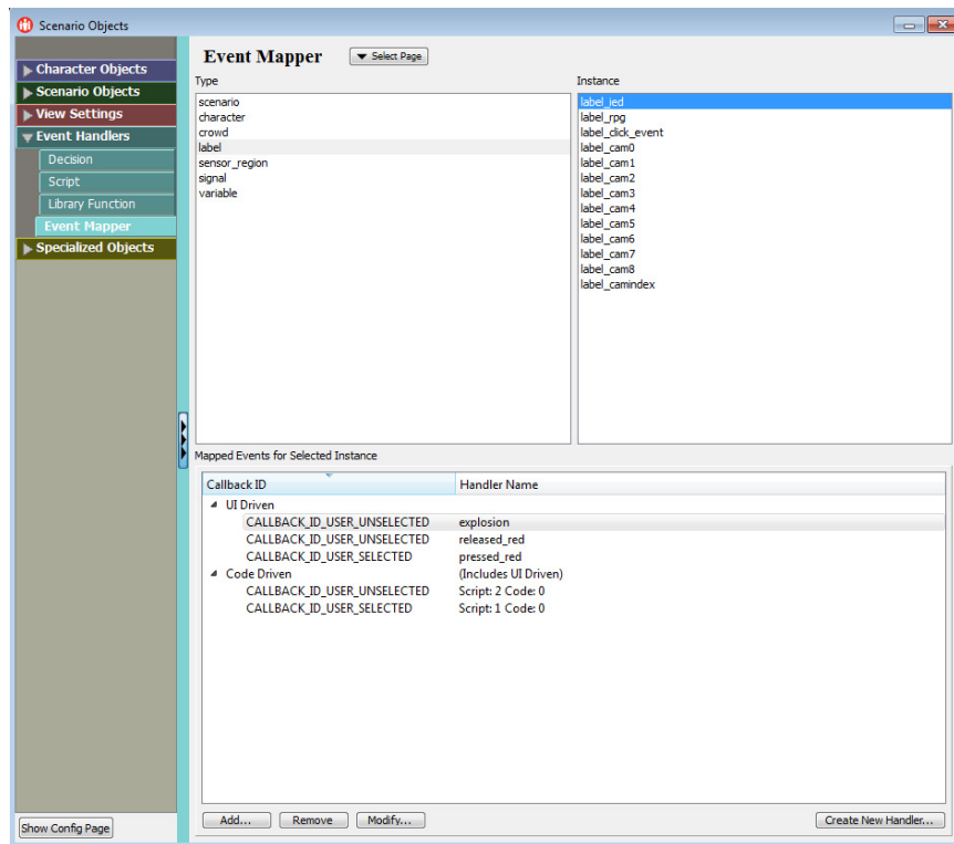
Figure 10-6. Event Mapper page
