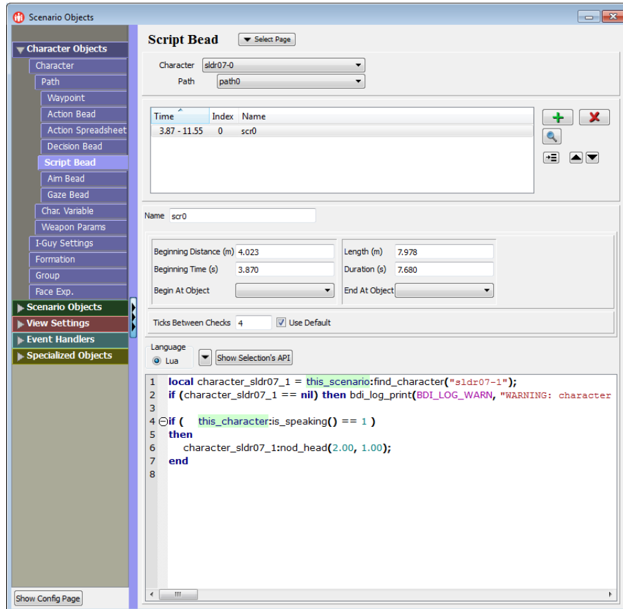
Figure 7-8. Script Bead page
