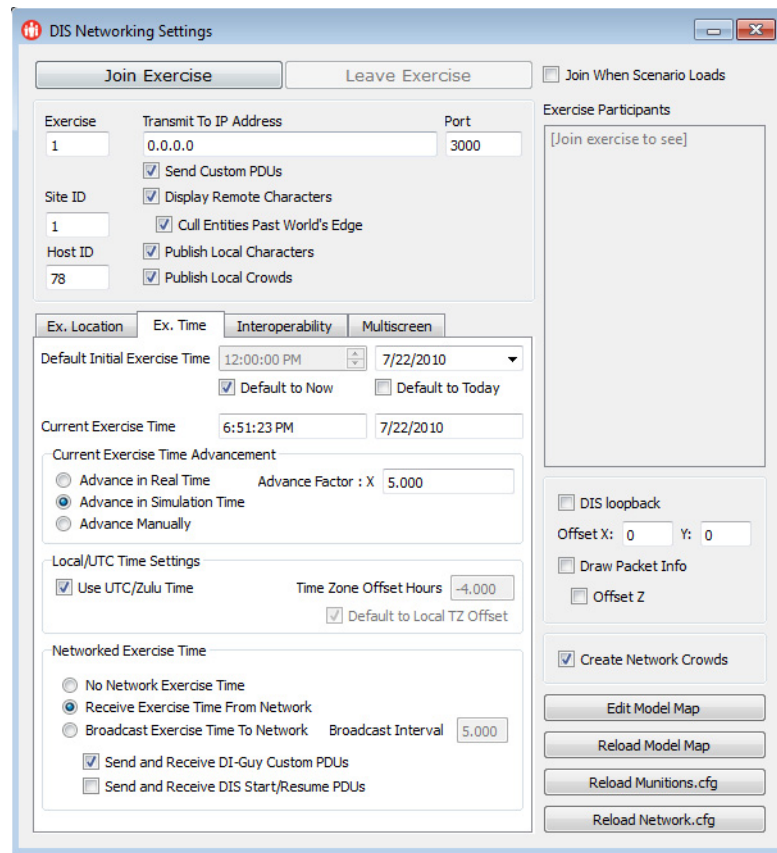
Figure 14-1. DIS Networking Settings dialog box
