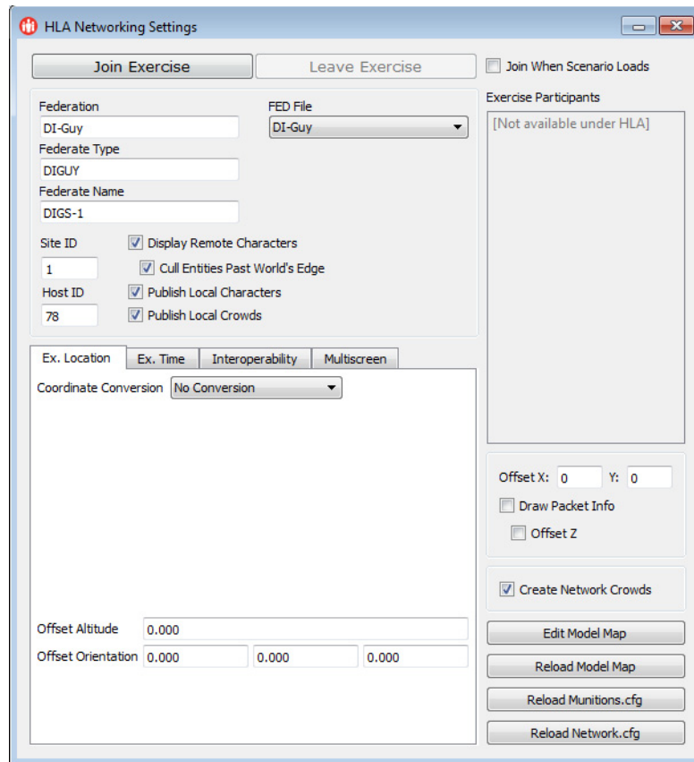
Figure 14-3. HLA Networking Settings dialog box
