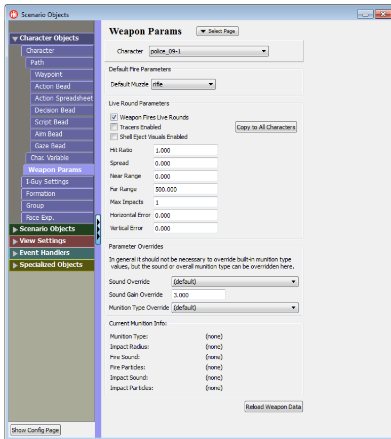
Figure 5-5. Weapon Params page
