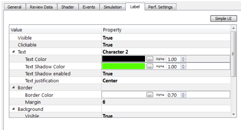
Figure 5-13. Label Tab Advanced UI
