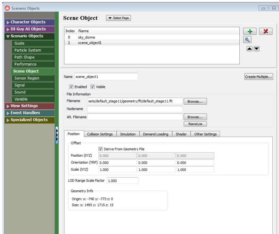
Figure 12-2. Scene Object page
