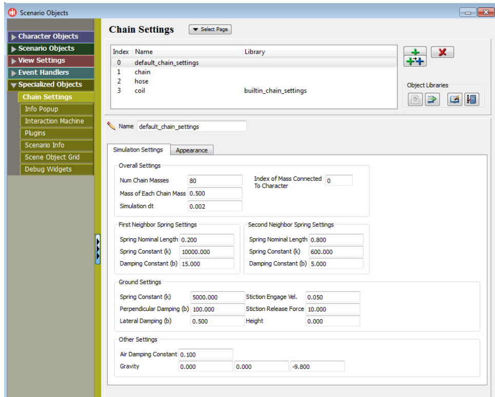
Figure 5-14. Chain Settings page
