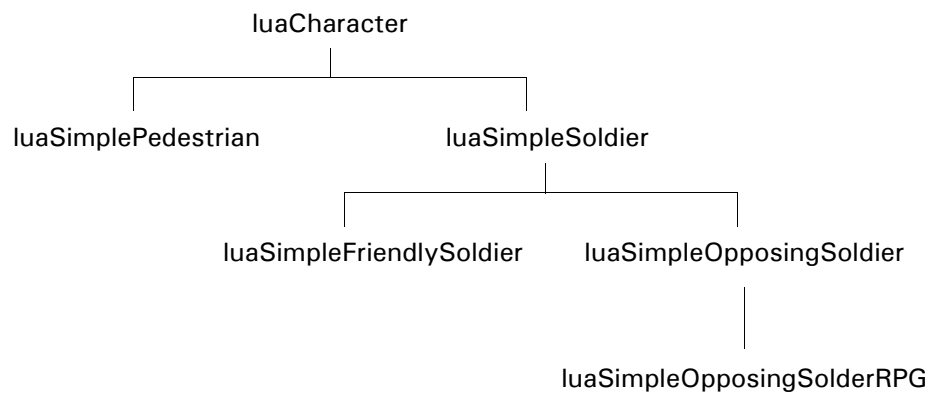
Figure 5-4. Class inheritance diagram for AI minds
