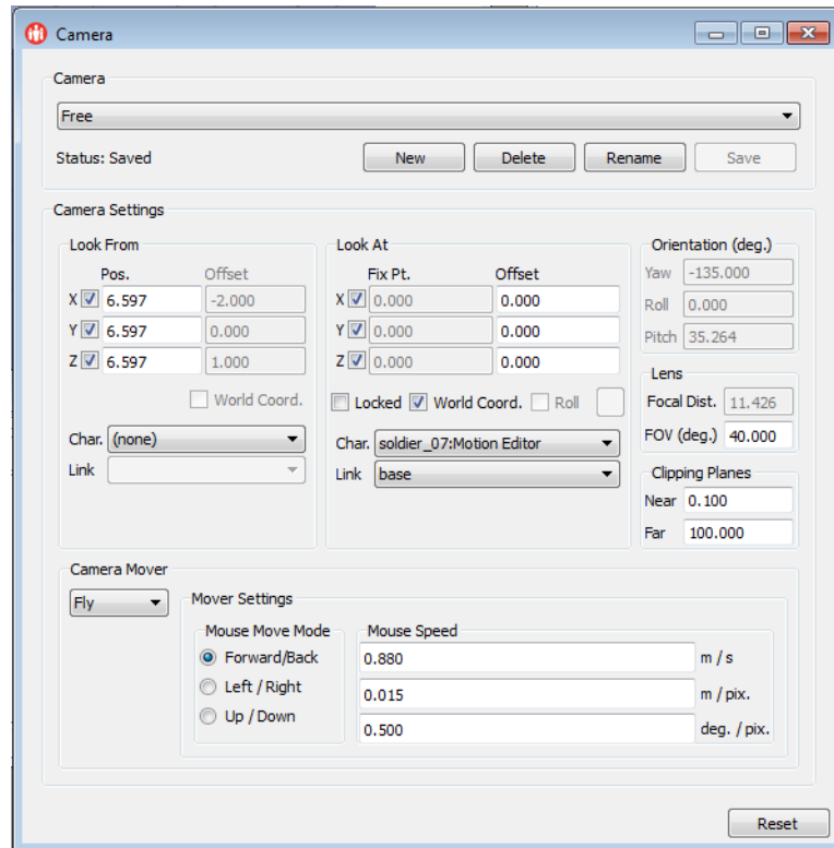
Figure 6-3. Camera dialog box
