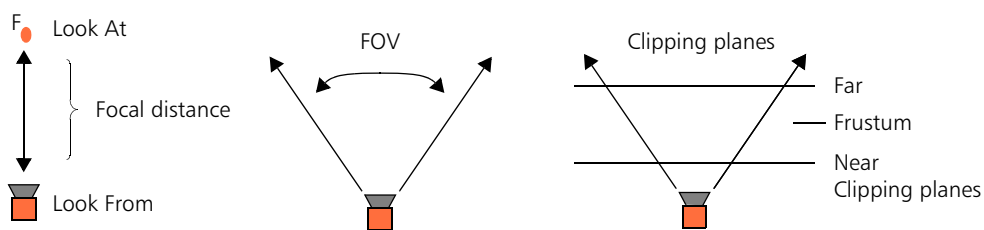
Figure 6-1. Look At, focal distance, FOV, clipping planes
