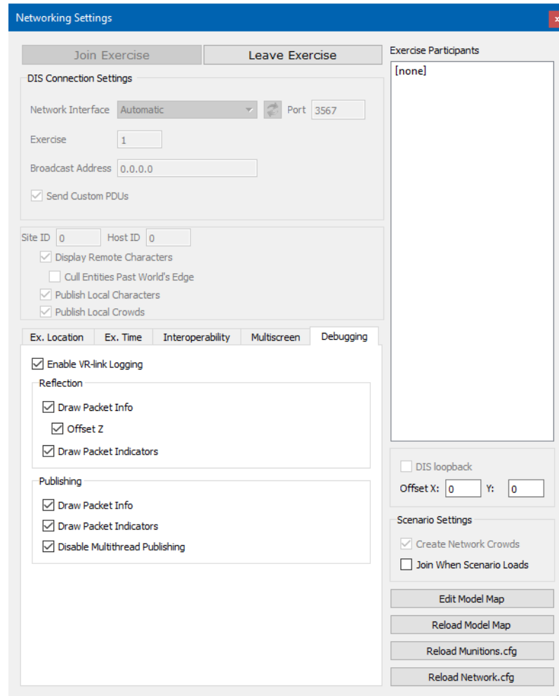
Figure 14-6. Network Settings, Debugging tab
