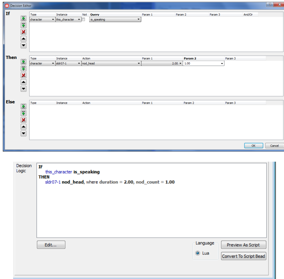
Figure 7-7. Decision Editor and finished decision logic
