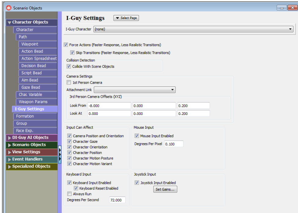
Figure 5-10. I-Guy Settings page
