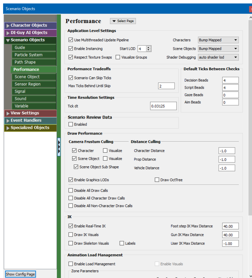
Figure 11-2. Scenario Objects:Performance page
