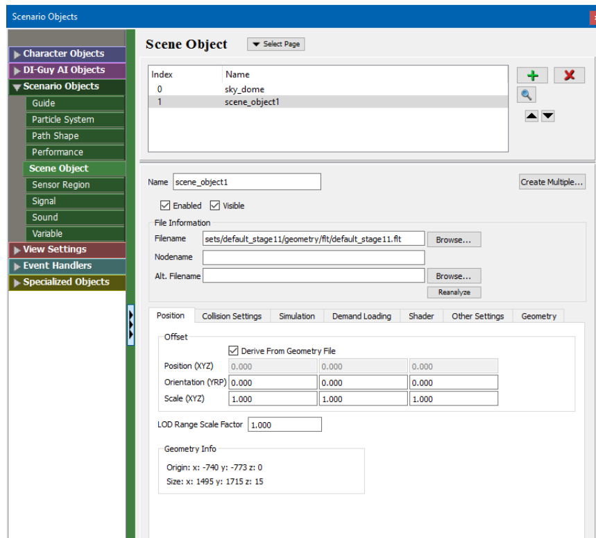
Figure 3-25. Scene Object page
