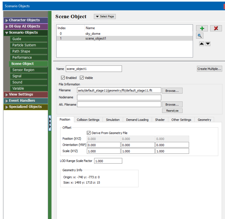
Figure 12-2. Scene Object page
