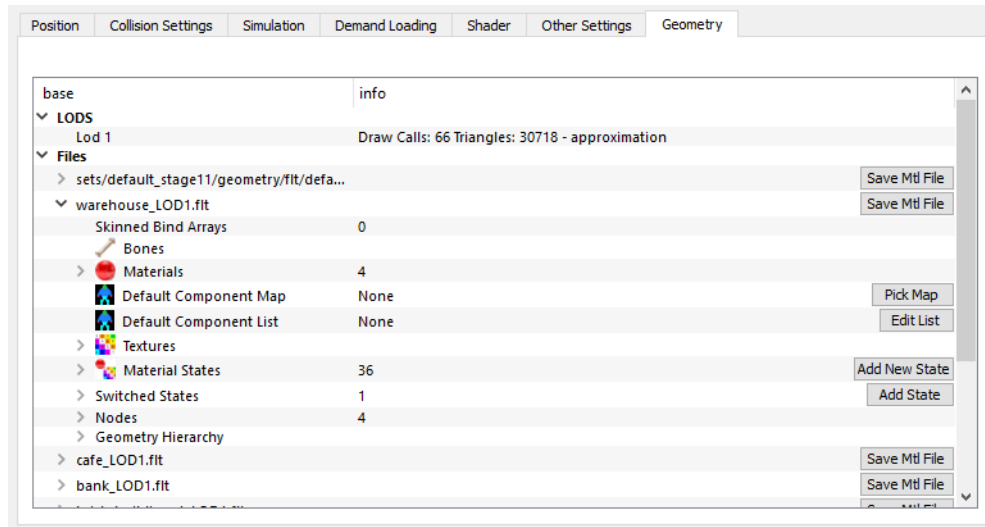
Figure 12-9. Scene Object page, Geometry tab
