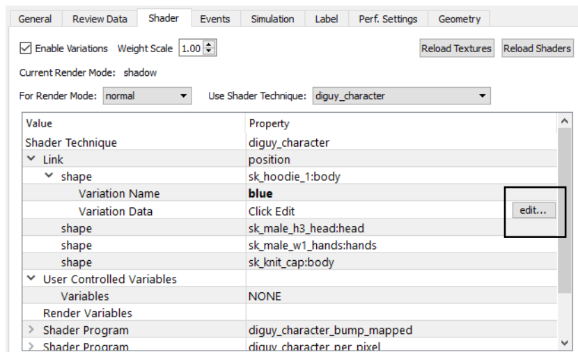
Figure 5-3. Character page, Shader tab
