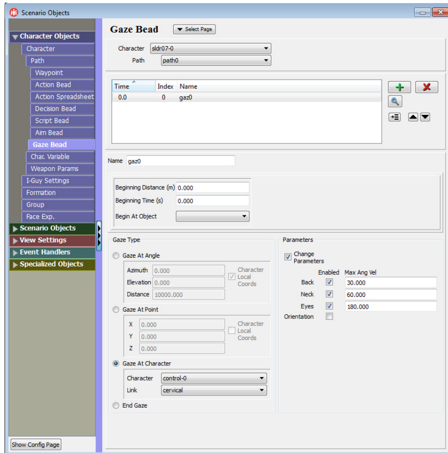
Figure 7-10. Gaze Bead page
