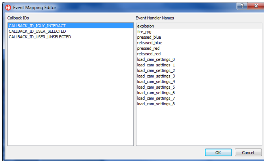
Figure 10-7. Event Mapping Editor
