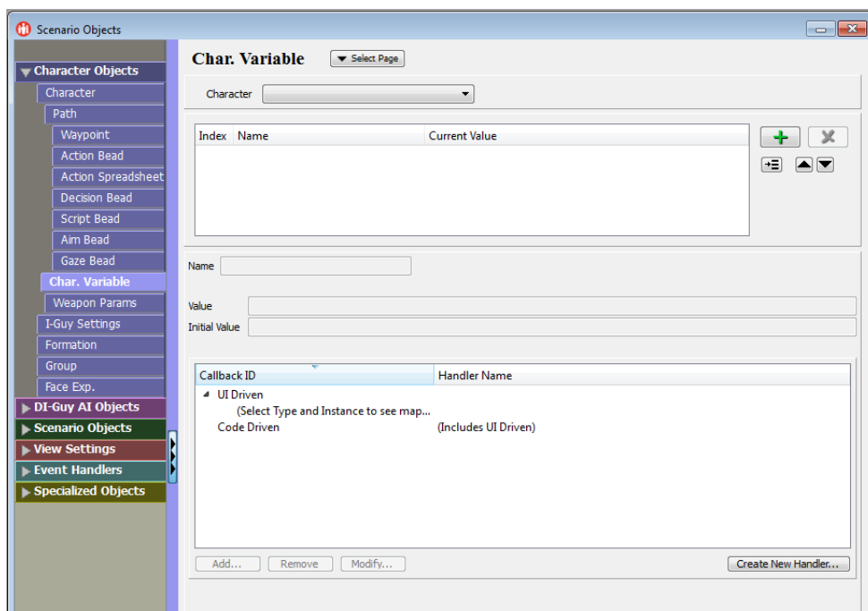
Figure 4-6. Character Variable page
