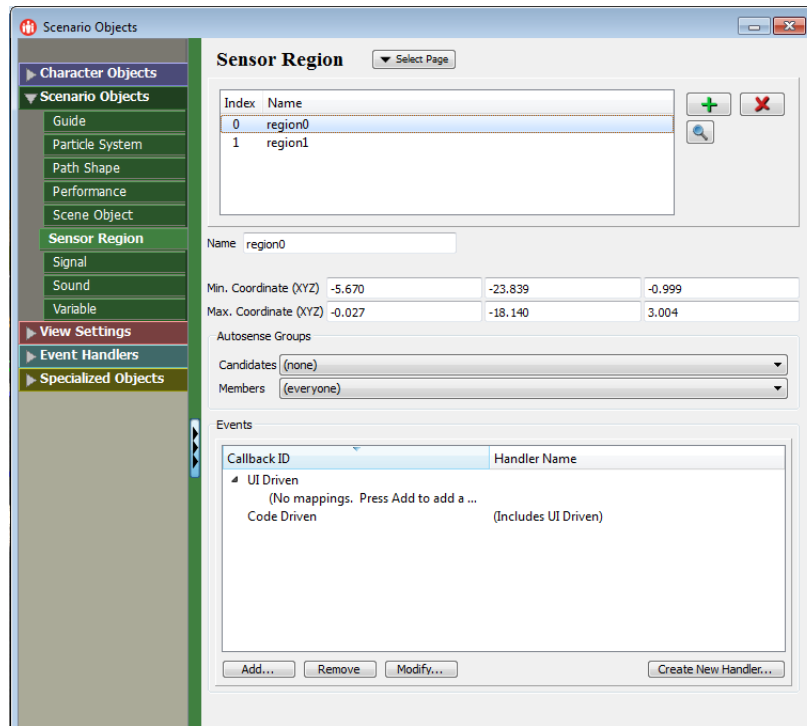
Figure 8-6. Sensor Region page
