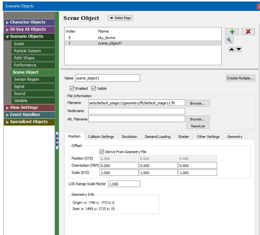
Figure 11-4. Scene Object page
