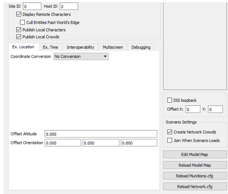
Figure 12-3. Ex. Location tab
