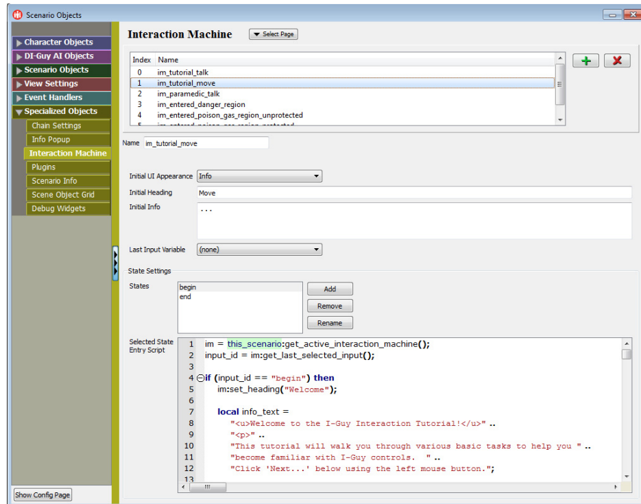
Figure 10-14. Interaction Machine page
