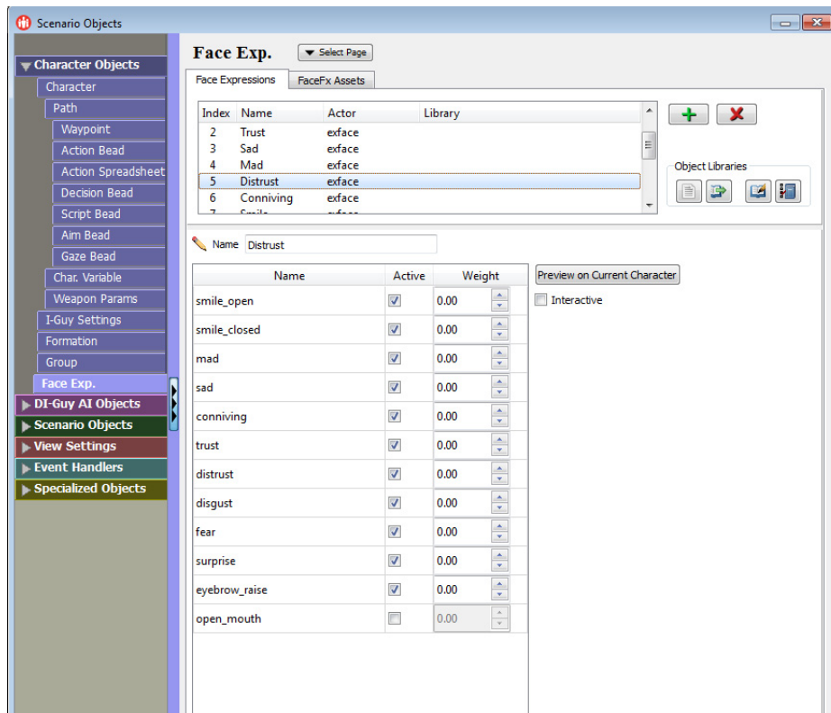
Figure 5-12. Face Exp. page
