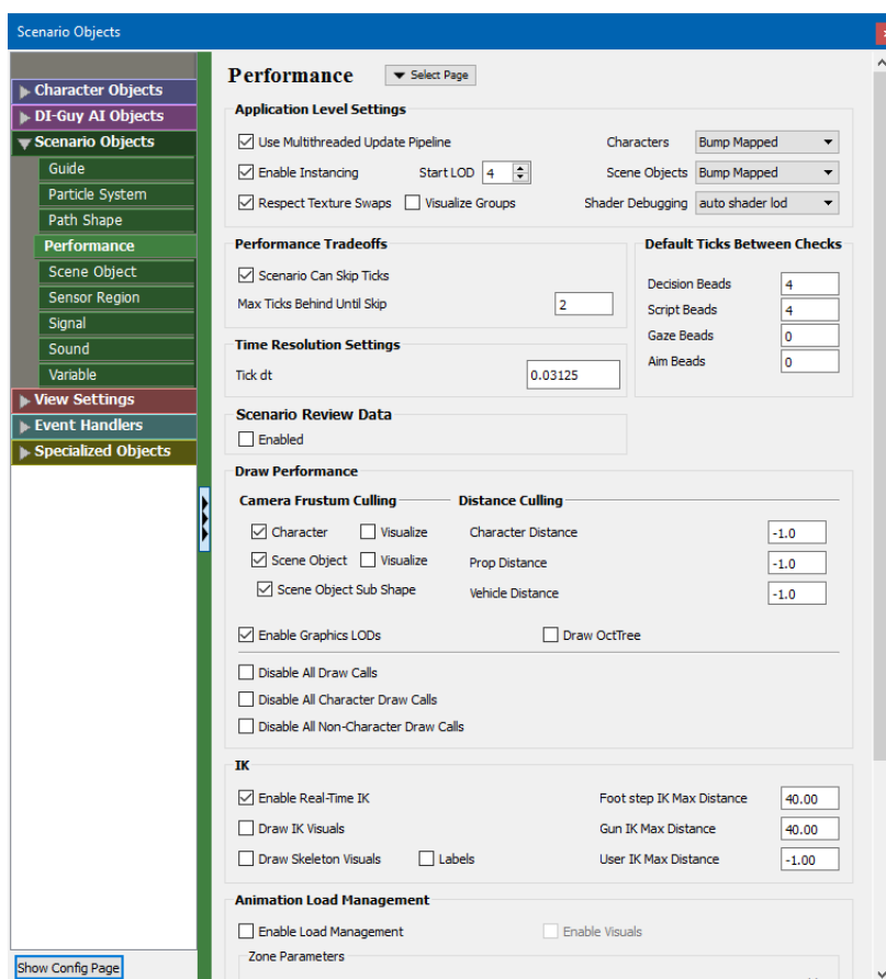
Figure 11-2. Scenario Objects:Performance page
