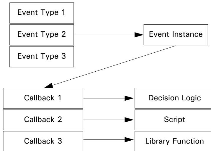
Figure 10-1. Events and event mapping
