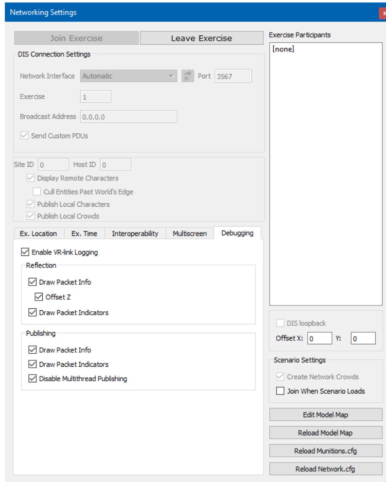
Figure 14-6. Network Settings, Debugging tab
