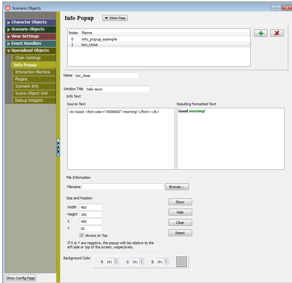
Figure 10-12. Info Popup page
