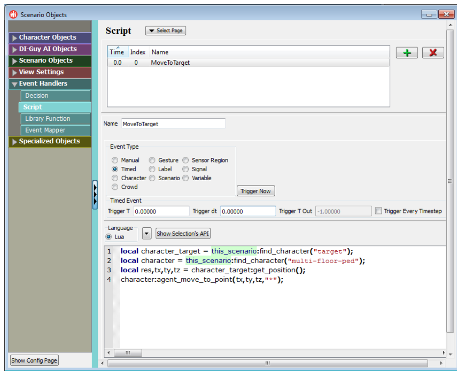
Figure 3-28. MoveToTarget script
