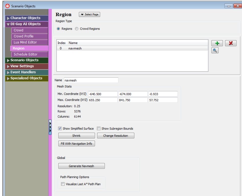
Figure 7-2. Region page
