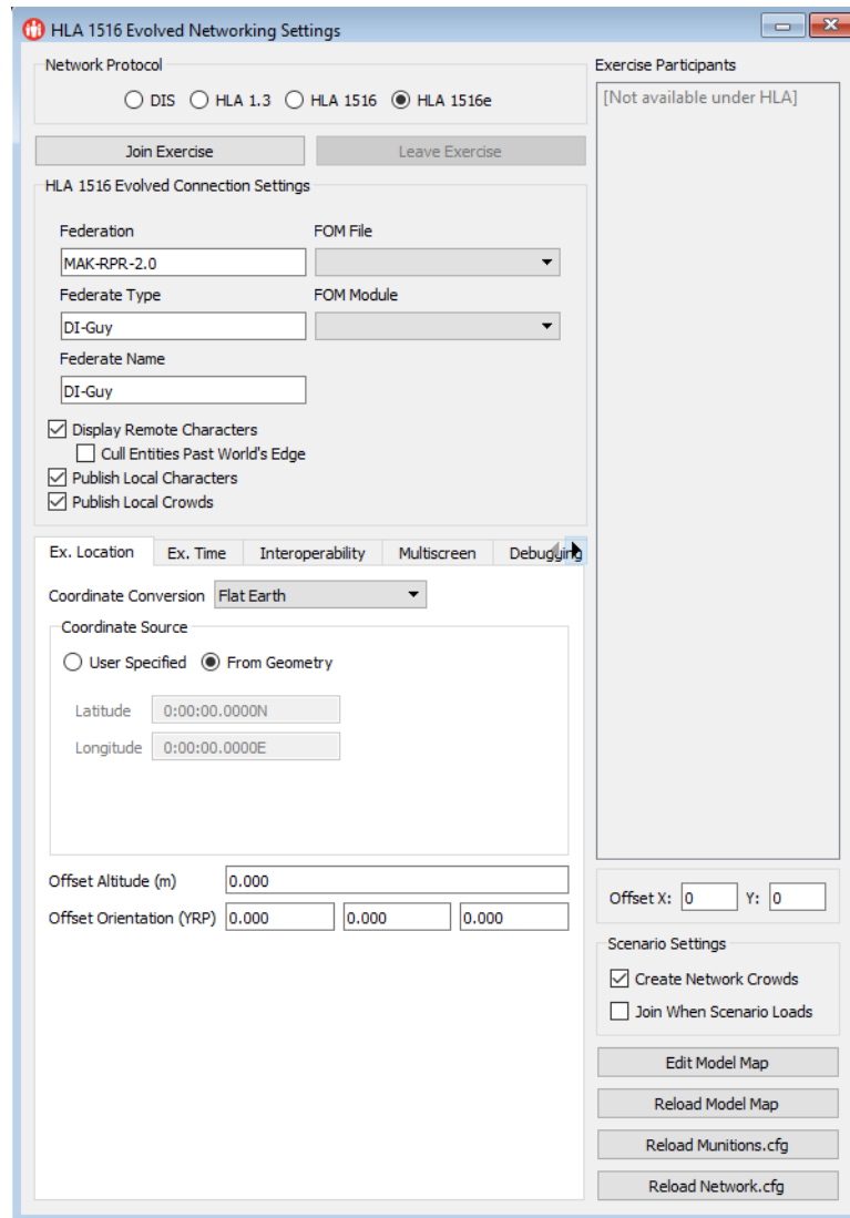
Figure 14-3. Networking Settings dialog box for HLA Evolved
