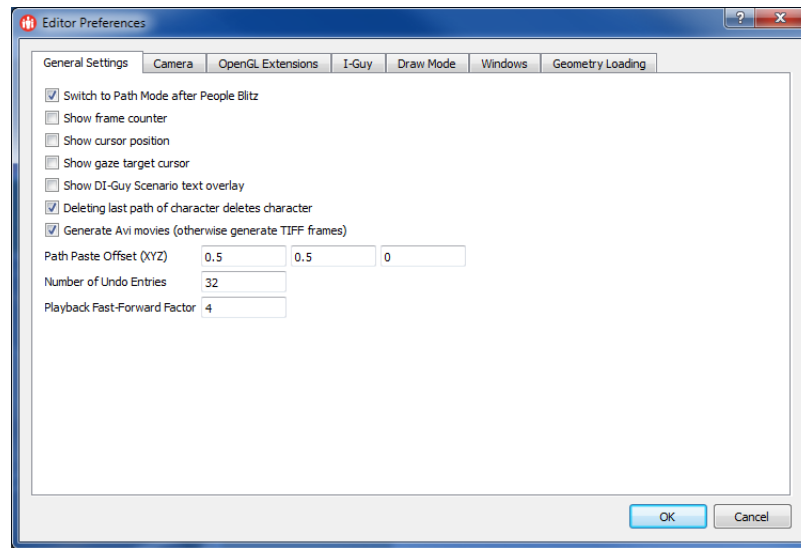
Figure 12-6. Editor Preferences, General Settings
