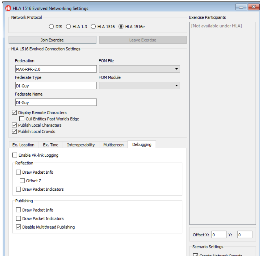
Figure 14-6. Network Settings, Debugging tab
