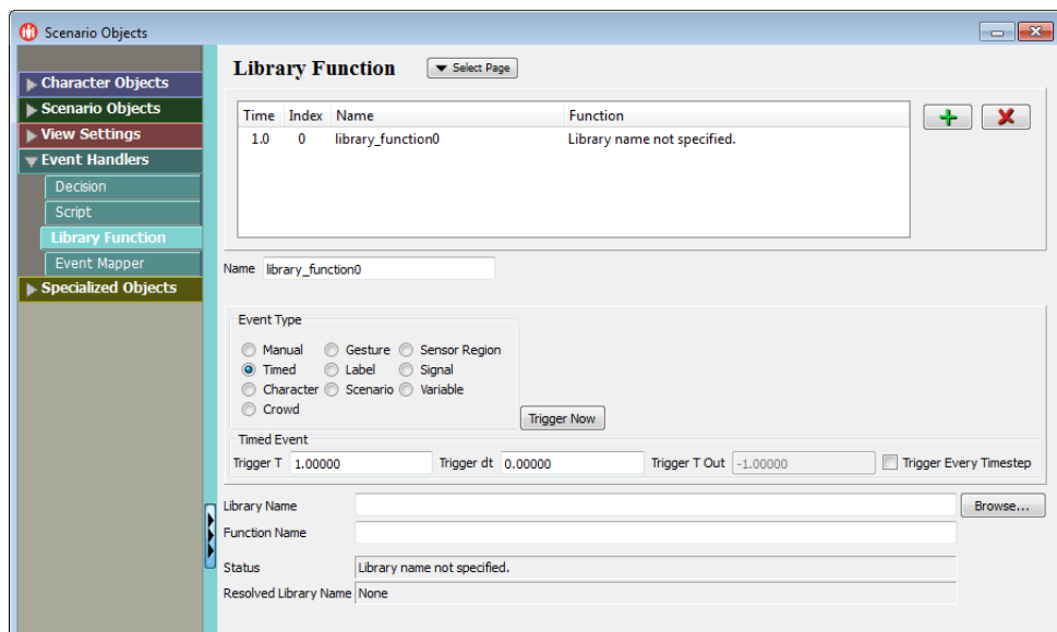
Figure 10-5. Library Function page
