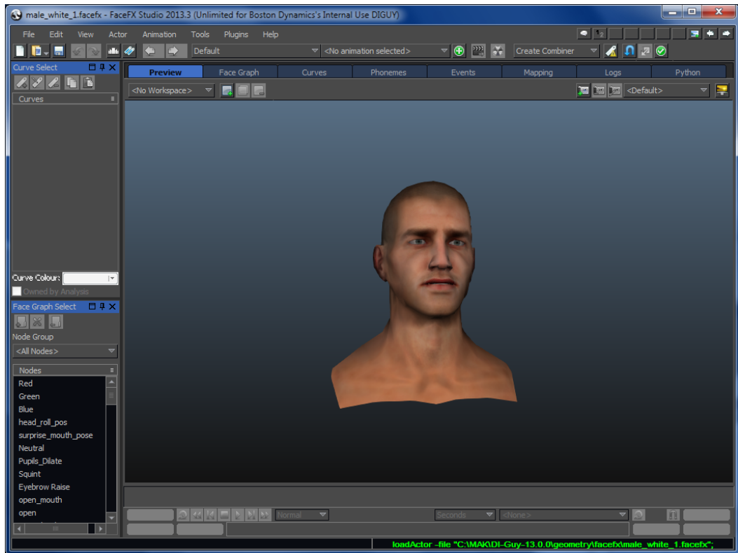
Figure 11. FaceFX
