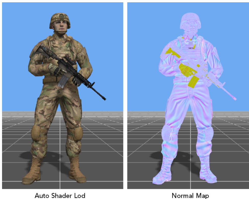
Figure 28. Shader debugging
