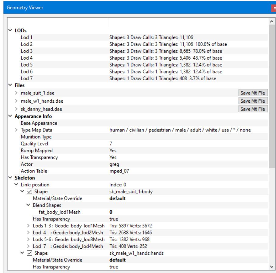
Figure 3. Geometry Overview window
