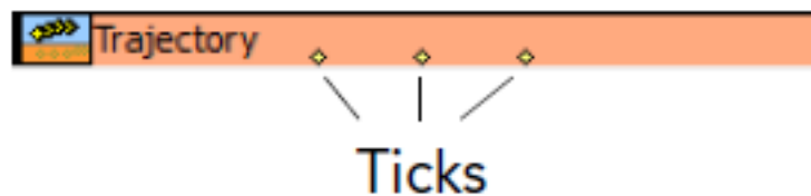
Figure 33. Trajectory containing atoms
