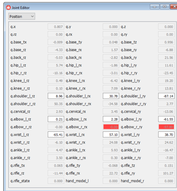
Figure 20. Joint Editor with left arm joints active
