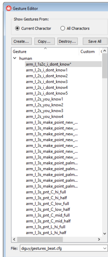
Figure 79. Gestures and gesture tables list
