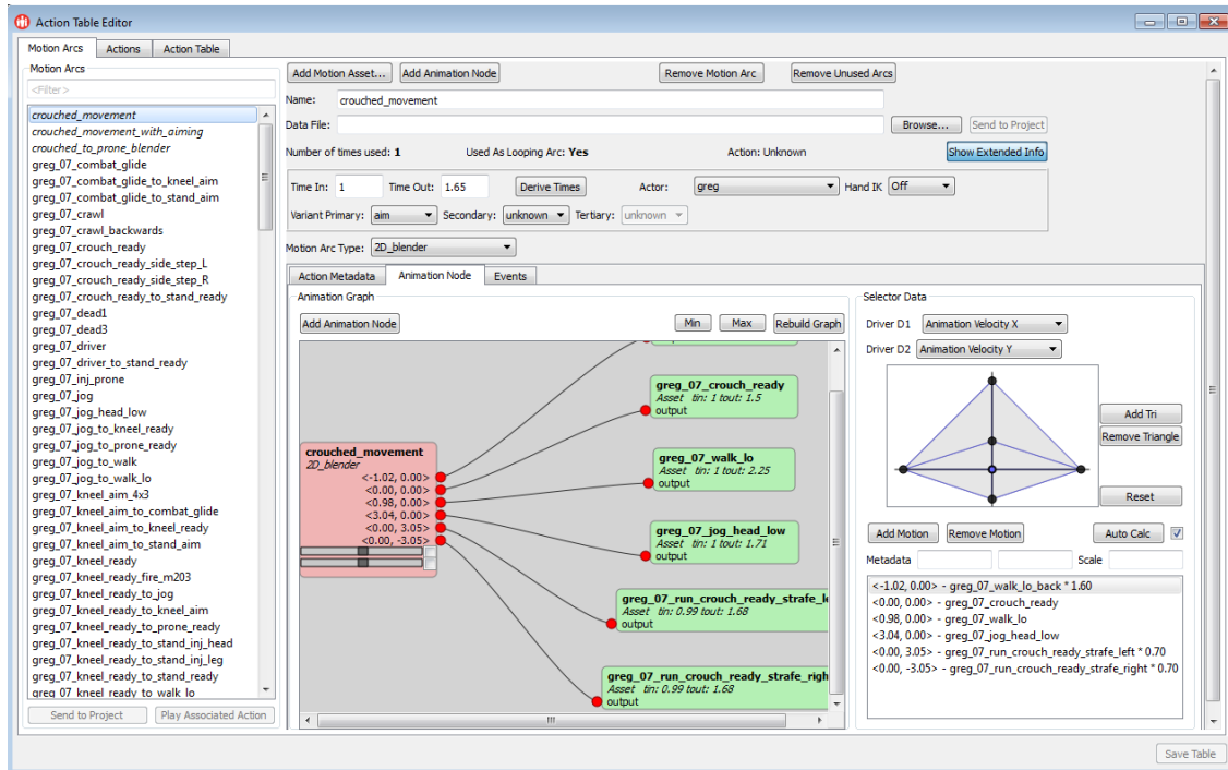
Figure 73. Motion Arcs tab
