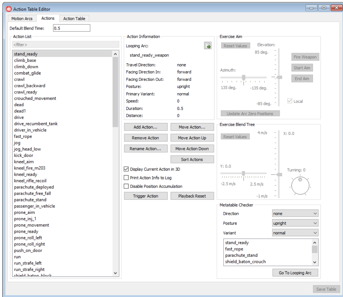
Figure 64. The Action Table Editor
