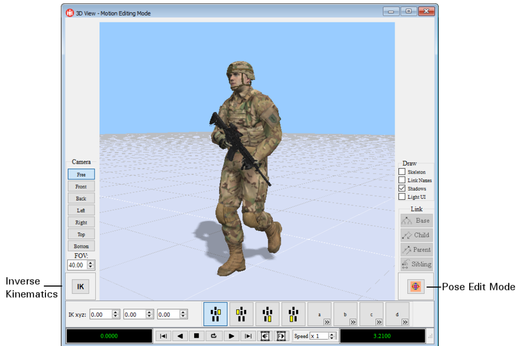
Figure 12. 3D View
