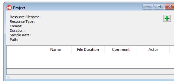
Figure 5. Project window
