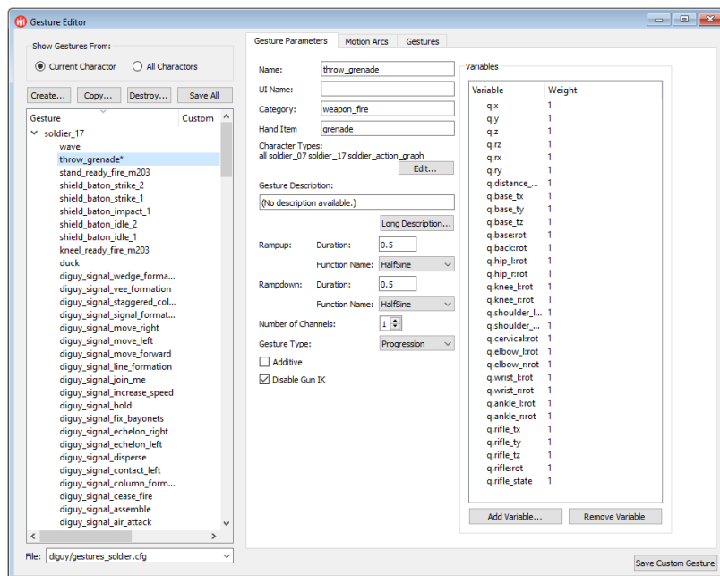
Figure 78. The Gesture Table Editor
