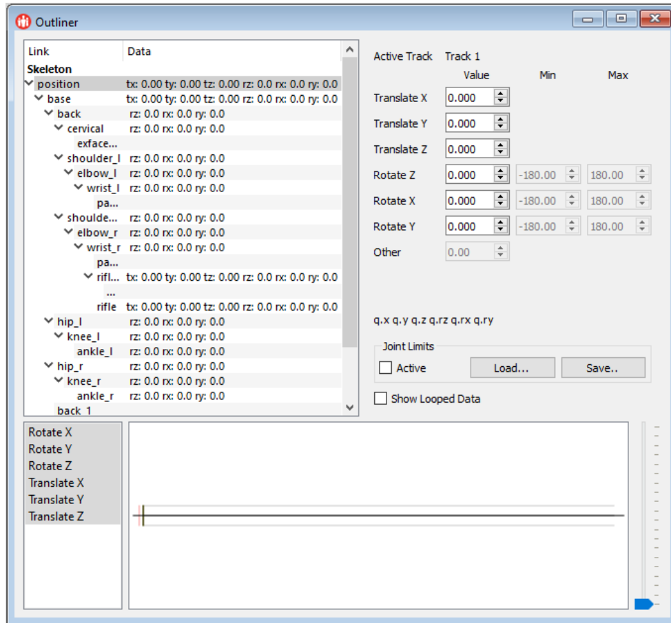
Figure 53. The Outliner
