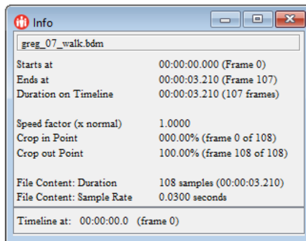
Figure 51. Info window
