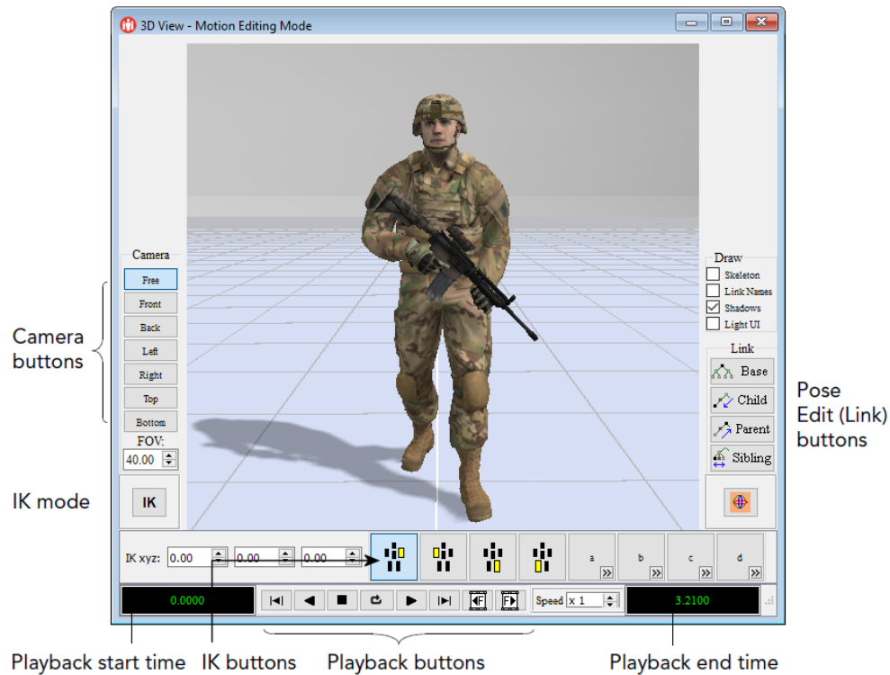
Figure 25. 3D View
