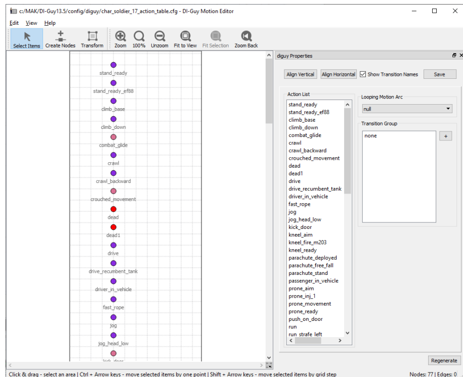
Figure 77. New graph
