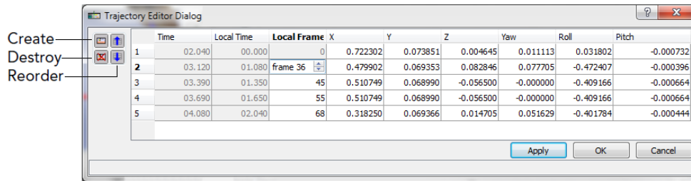
Figure 35. Trajectory Editor
