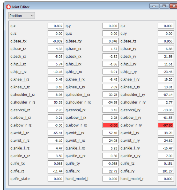
Figure 18. Joint Editor
