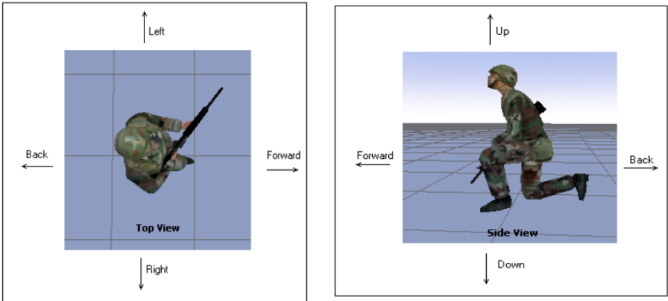
Figure 74. Direction types
