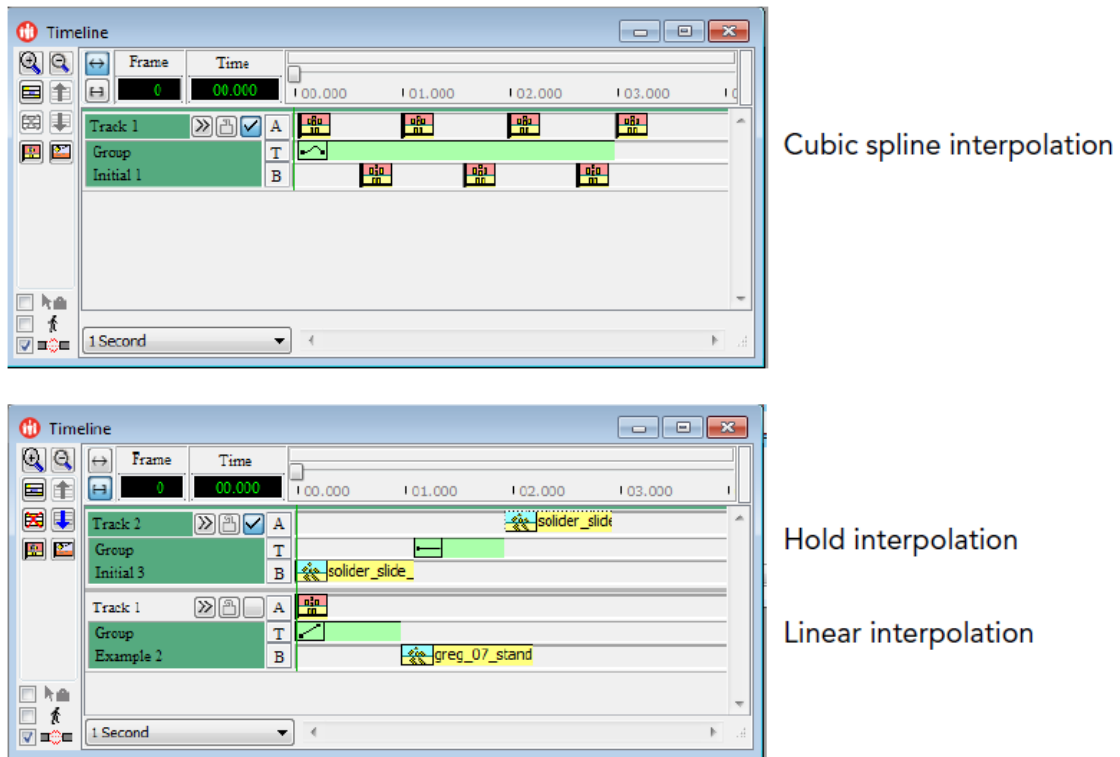
Figure 45. Interpolation transitions
