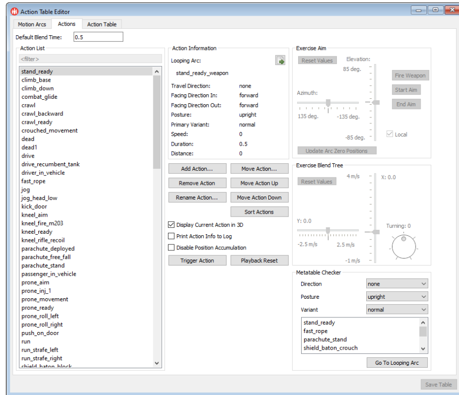
Figure 3. Action Table Editor, Actions tab
