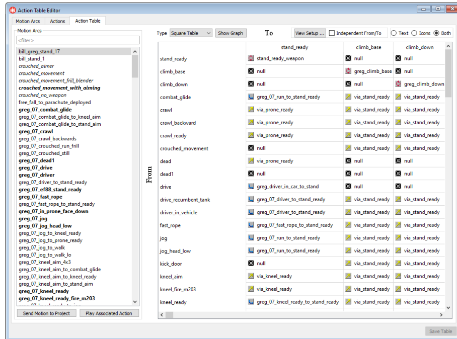
Figure 4. Action Table Editor, Action Table tab
