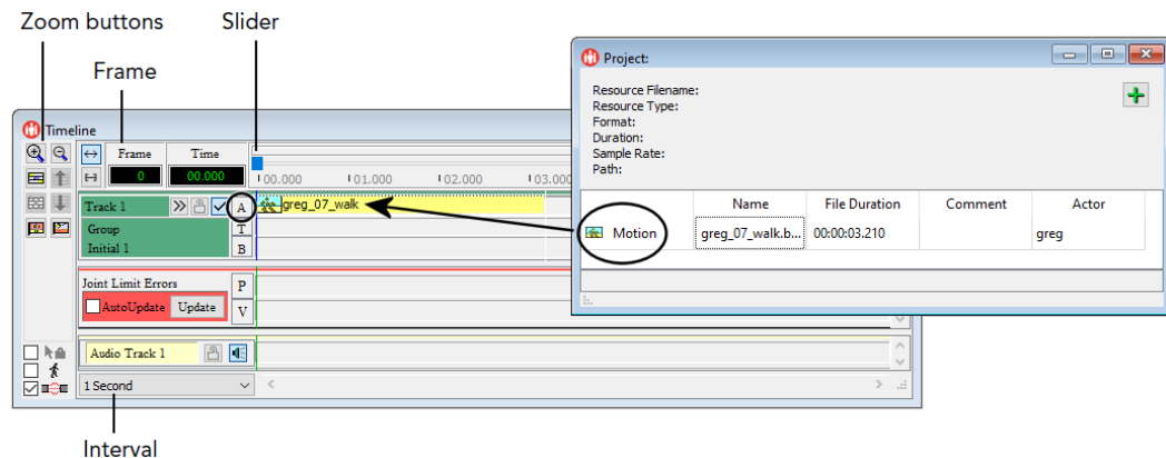
Figure 10. Timeline window with motion added
