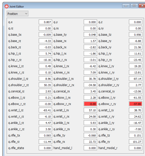
Figure 52. Joint Editor
