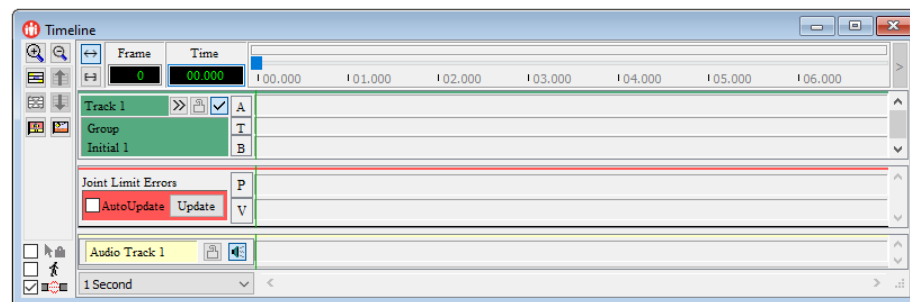
Figure 6. Timeline window
