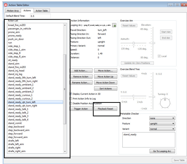
Figure 2-2. Action Table Editor, Actions tab
