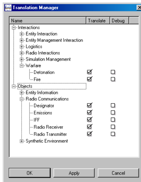
Figure 3-4. Translation Manager
