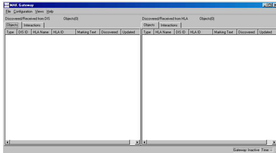
Figure 3-1. Gateway window
