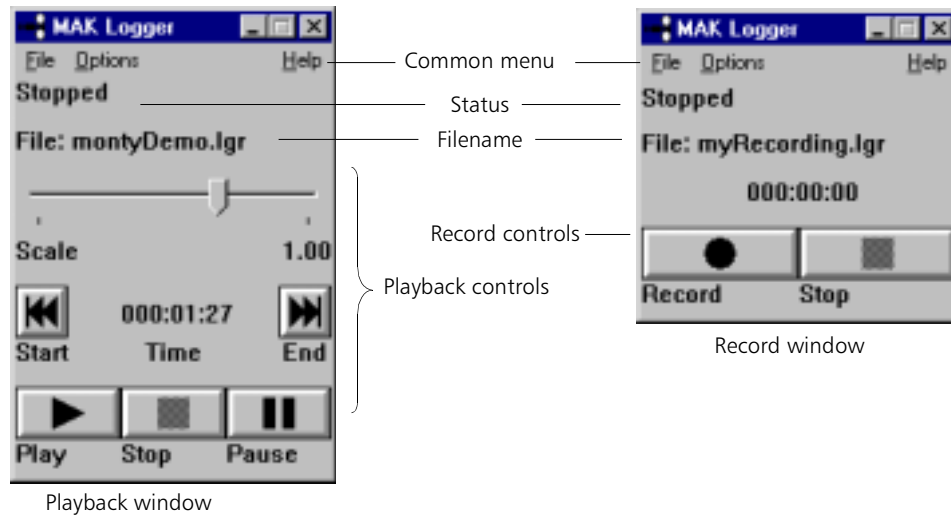
Figure 4-1. The Logger windows
