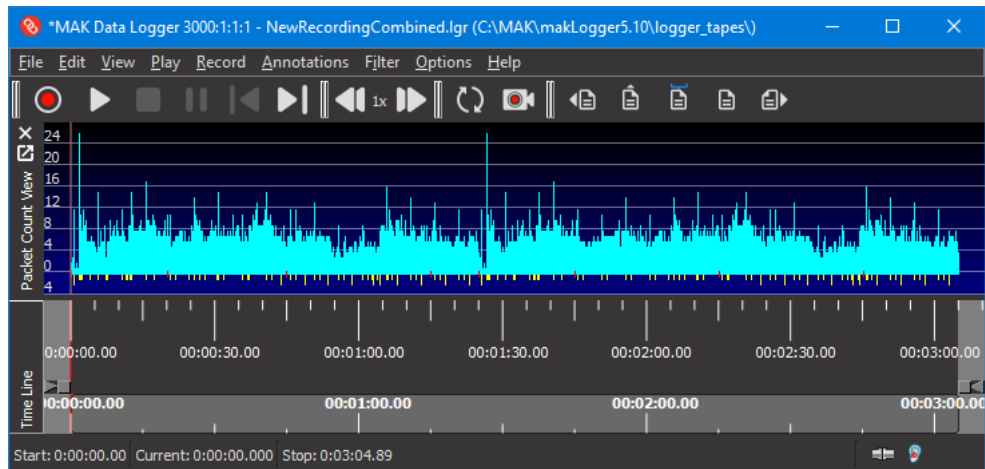
Figure 17. Packets deleted
