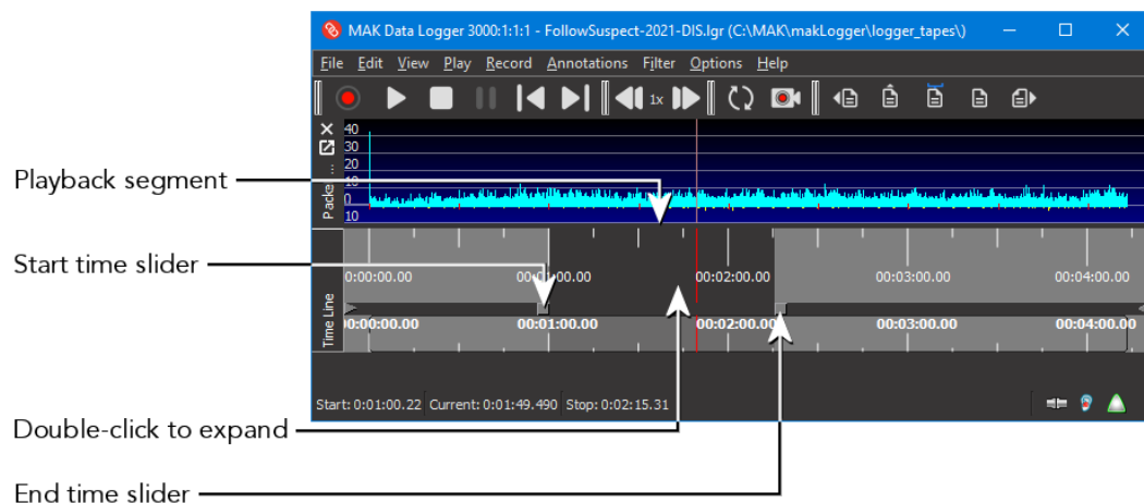
Figure 5. Timeline sliders
