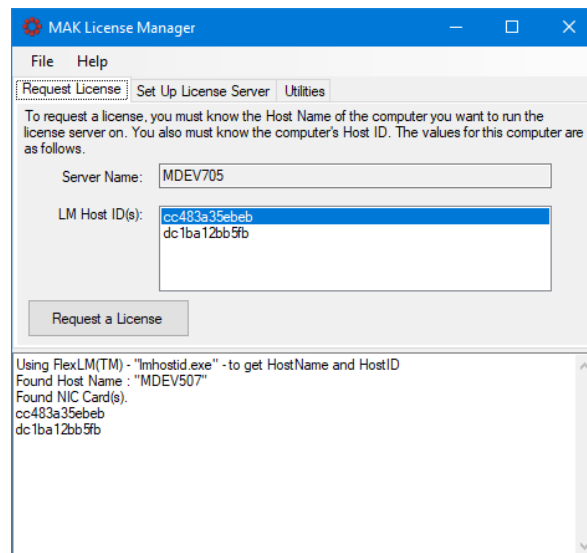
Figure 18. License Manager
