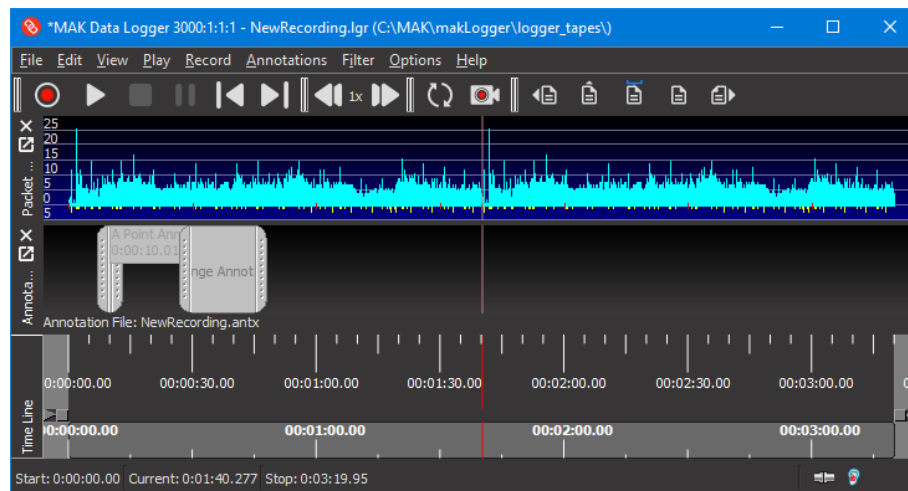
Figure 13. Concatenated files
