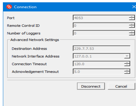
Figure 82. Connection dialog box
