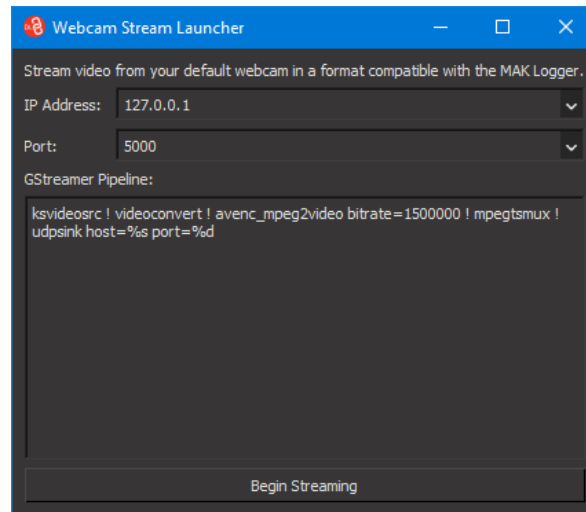
Figure 28. Webcam Stream Launcher
