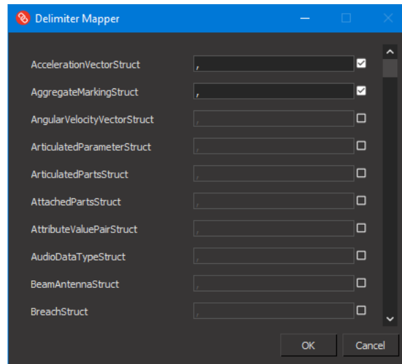
Figure 54. Delimiter Mapper dialog box
