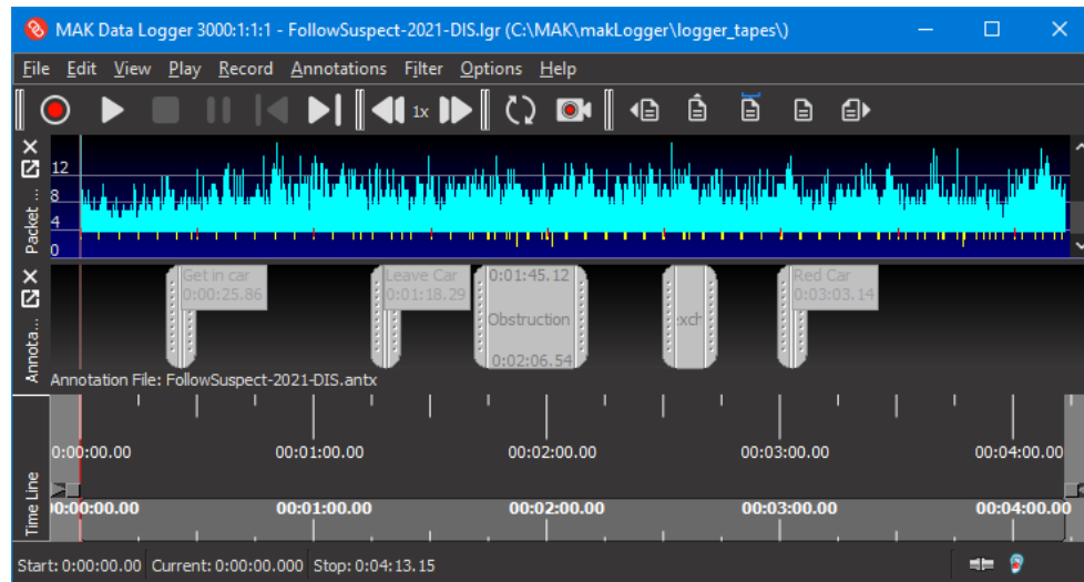
Figure 8. Connection status
