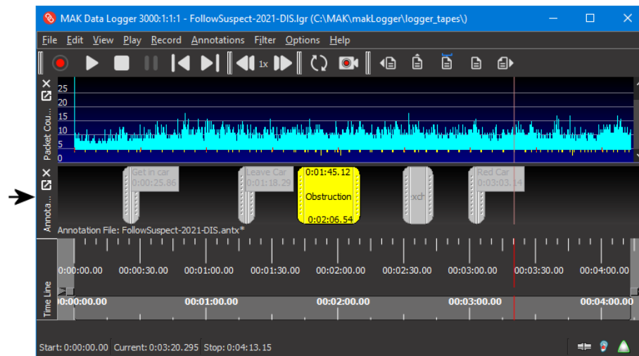
Figure 39. Annotations display
