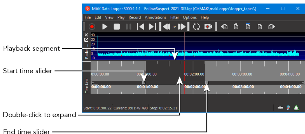
Figure 29. Timeline sliders
