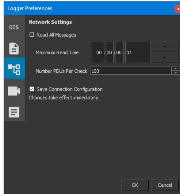
Figure 15. Logger Preferences dialog box, Network Settings page
