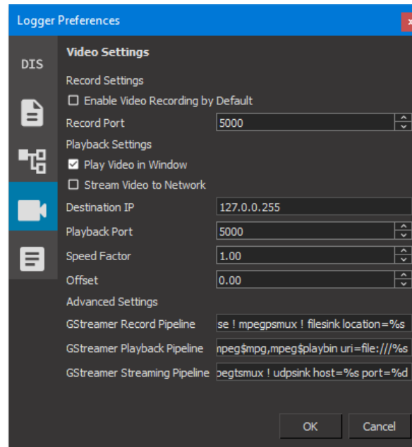
Figure 16. Video Settings page
