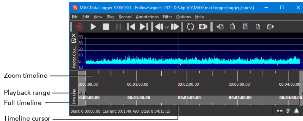
Figure 19. Timeline
