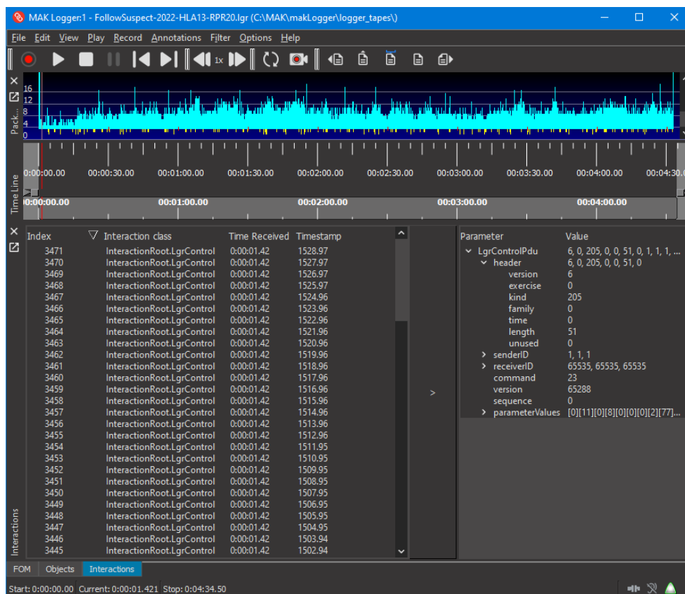
Figure 52. Interactions tab
