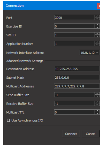
Figure 9. Connection dialog box for DIS
