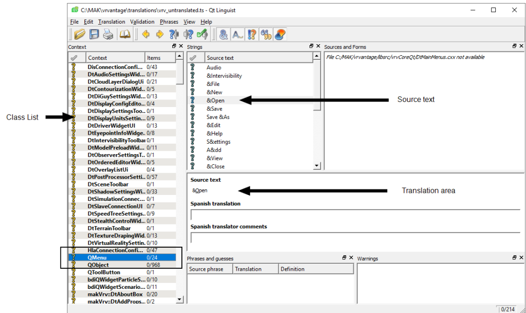
Figure 4. Linguist window
