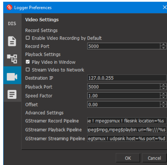
Figure 16. Video Settings page
