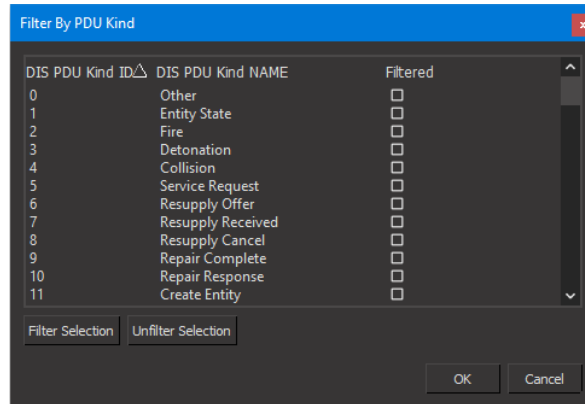
Figure 44. Filter By PDU Kind dialog box
