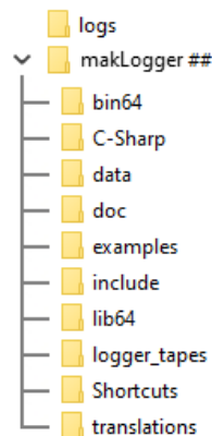
Figure 2. Logger directory structure
