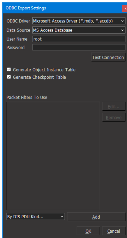
Figure 59. ODBC Export Settings dialog box (DIS)
