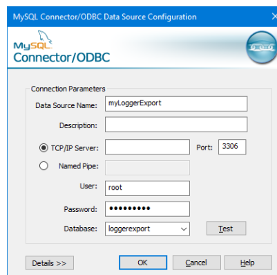
Figure 69. MySQL Connector/ODBC Data Source Configuration dialog box
