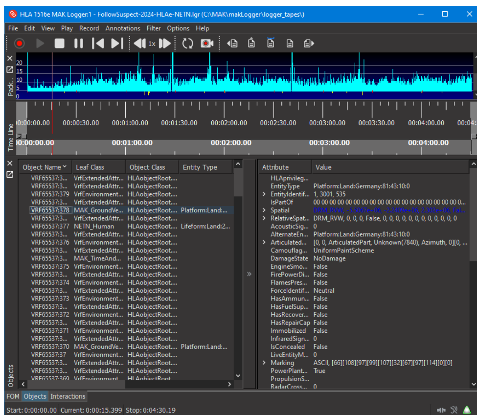
Figure 51. Objects tab
