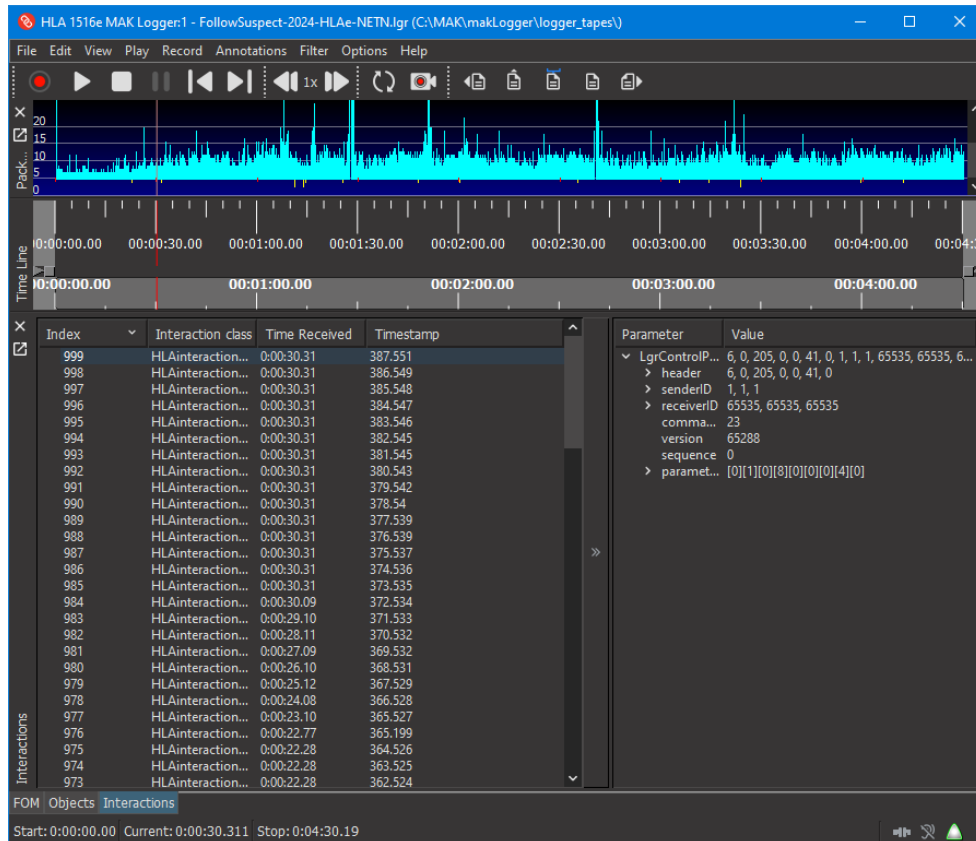
Figure 52. Interactions tab
