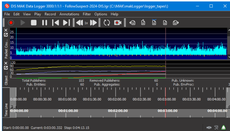
Figure 36. Object statistics
