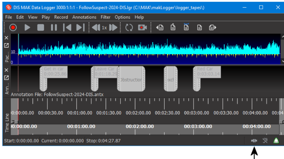
Figure 8. Connection status
