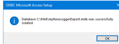
Figure 66. Information prompt
