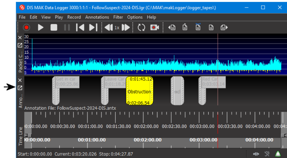
Figure 39. Annotations display
