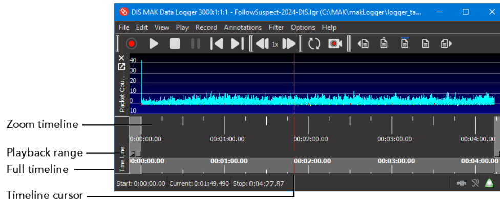
Figure 19. Timeline
