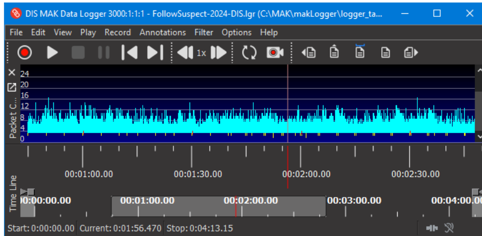
Figure 32. Zoomed timeline
