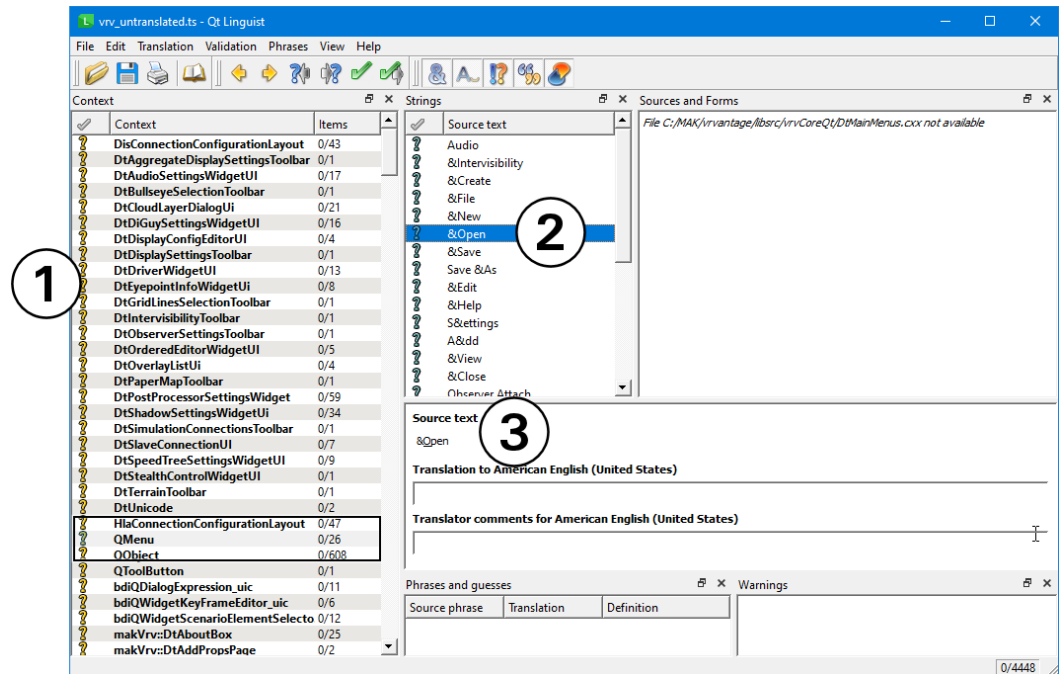
Figure 5. Linguist window
