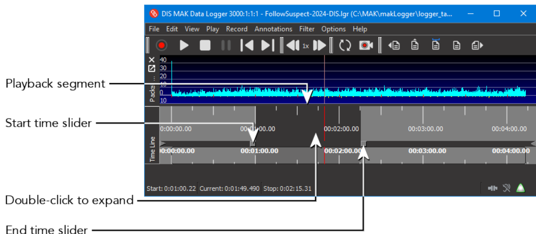
Figure 29. Timeline sliders
