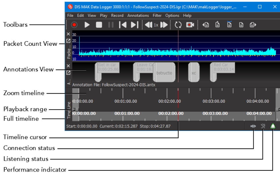
Figure 18. Logger window with a Logger file loaded
