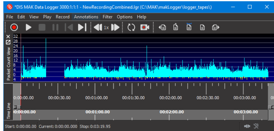
Figure 15. Packets cleared
