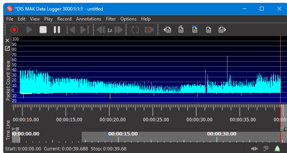
Figure 3. New recording
