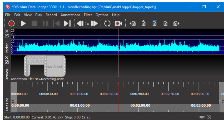
Figure 13. Concatenated files
