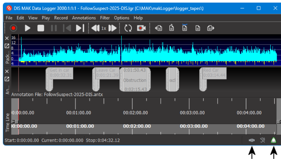
Figure 8. Connection status
