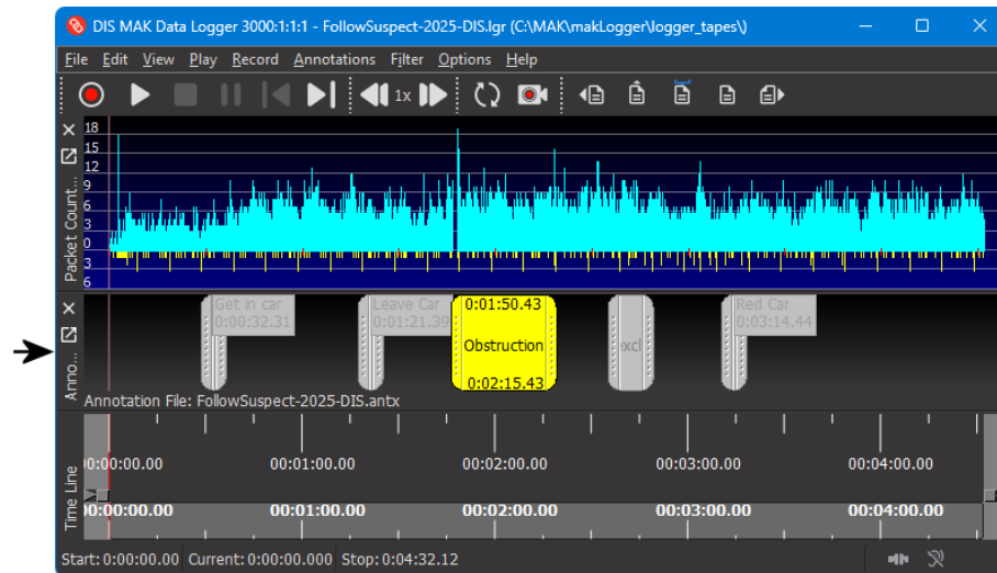
Figure 39. Annotations display
