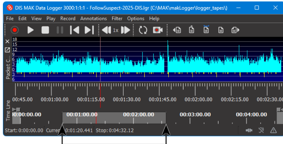
Figure 32. Zoomed timeline
