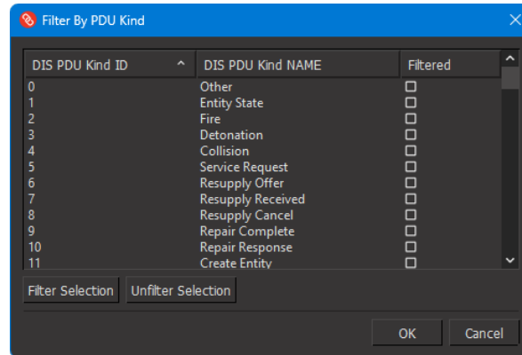
Figure 44. Filter By PDU Kind dialog box
