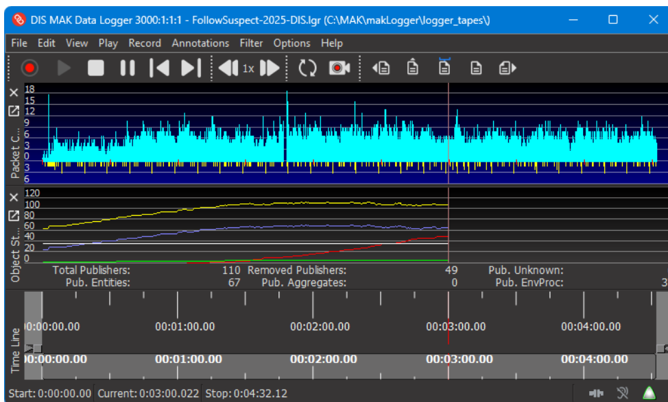
Figure 36. Object statistics
