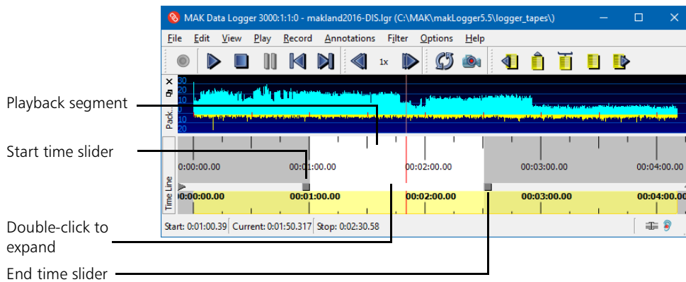
Figure 8-1. Timeline sliders
