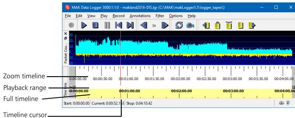
Figure 6-2. Timeline
