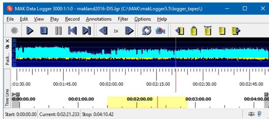
Figure 8-4. Zoomed timeline
