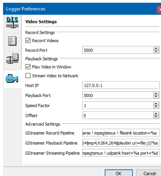
Figure 5-3. Video Settings page
