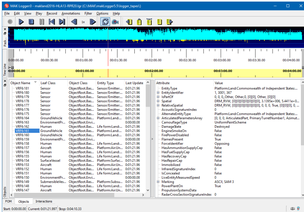
Figure 11-2. Objects tab
