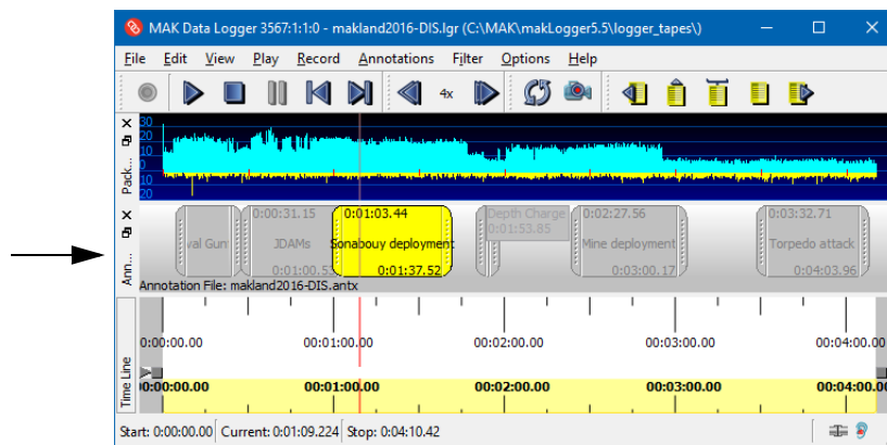
Figure 9-1. Annotations display
