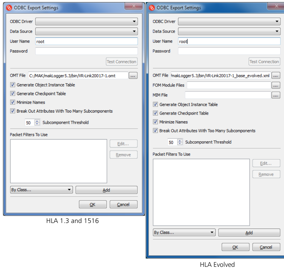
Figure 13-2. ODBC Export Settings dialog box (HLA)
