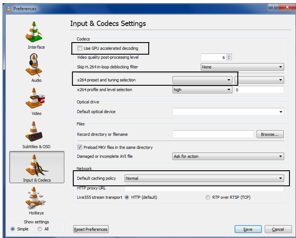
Figure 8-9. VLC Preferences, Inputs & Codecs
