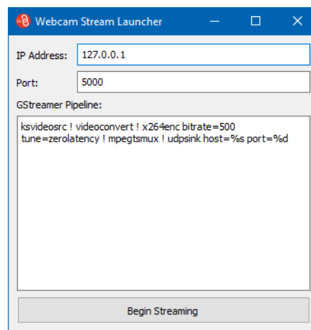
Figure 7-3. Webcam Stream Launcher
