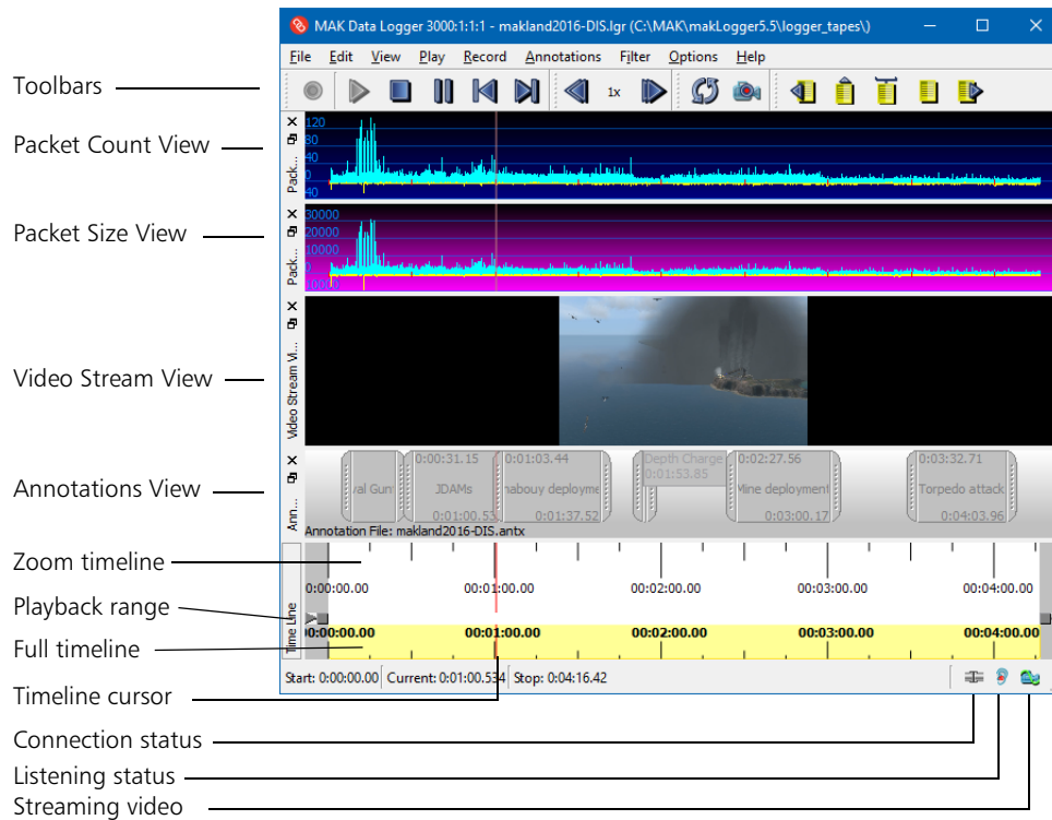
Figure 6-1. Logger window with a Logger file loaded
