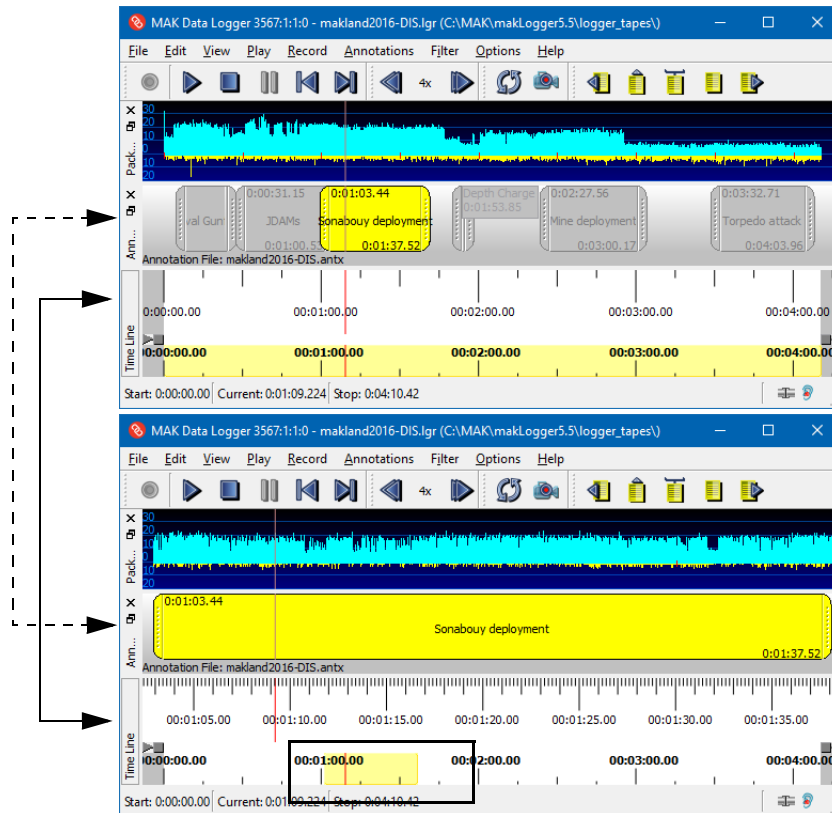
Figure 9-3. Zooming to an annotation
