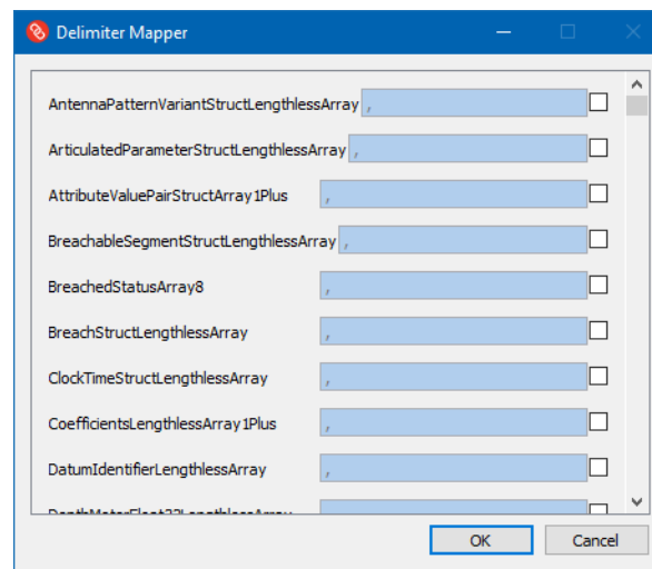
Figure 11-5. Delimiter Mapper dialog box
