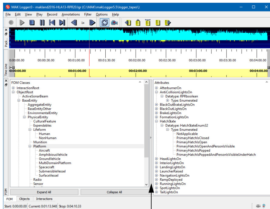
Figure 11-1. Traffic Analyzer, FOM tab
