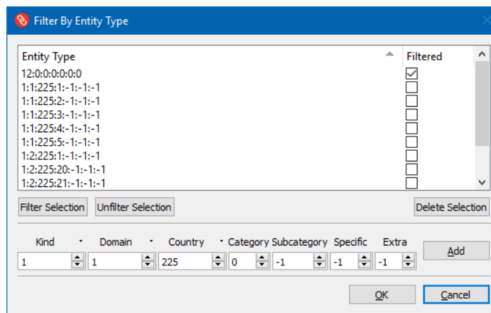
Figure 10-1. Filter By Entity Type dialog box
