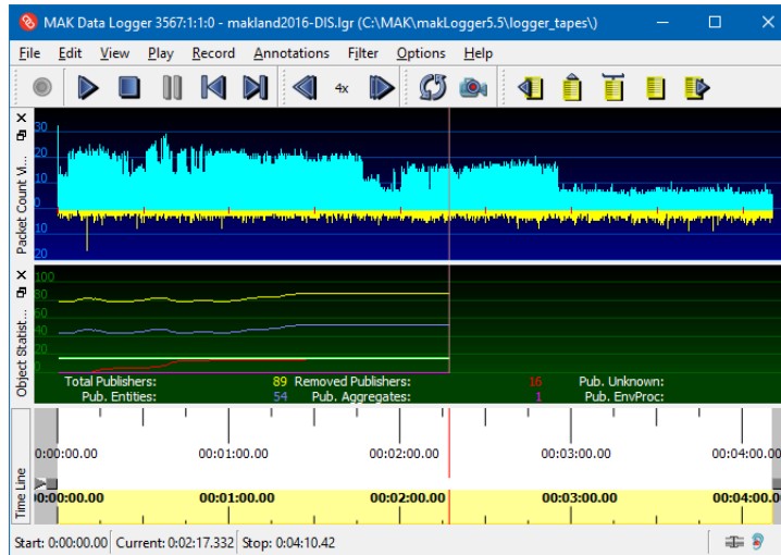
Figure 8-8. Object statistics
