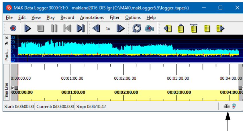
Figure 4-1. Connection status
