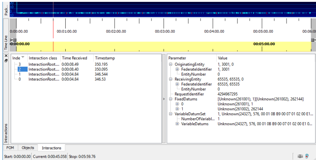
Figure 11-3. Interactions tab
