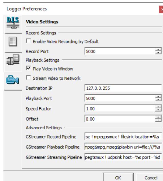
Figure 5-3. Video Settings page
