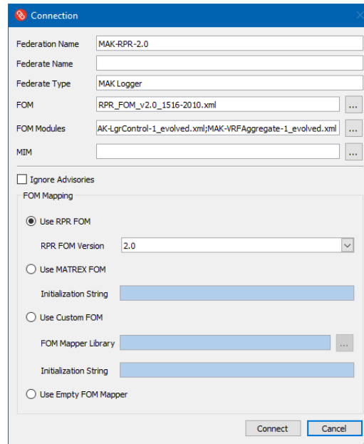
Figure 4-3. Connection dialog box for HLA Evolved
