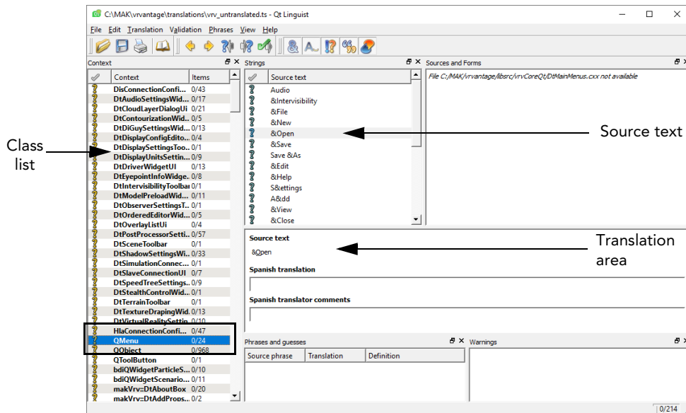
Figure 2-4. Linguist window
