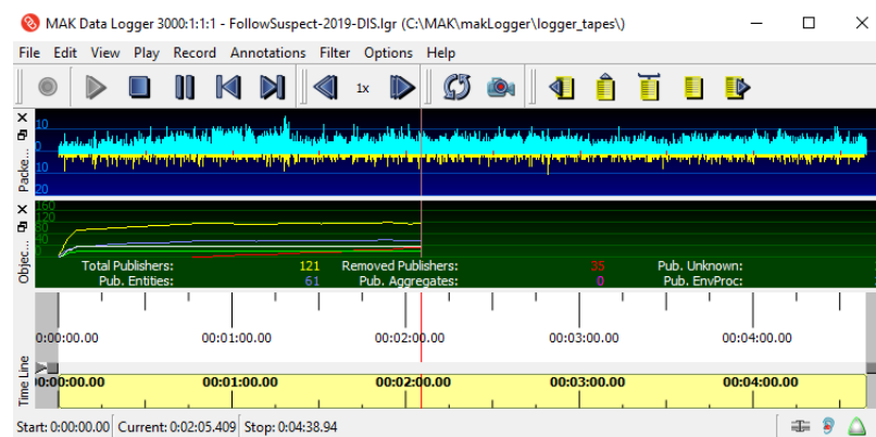
Figure 8-8. Object statistics
