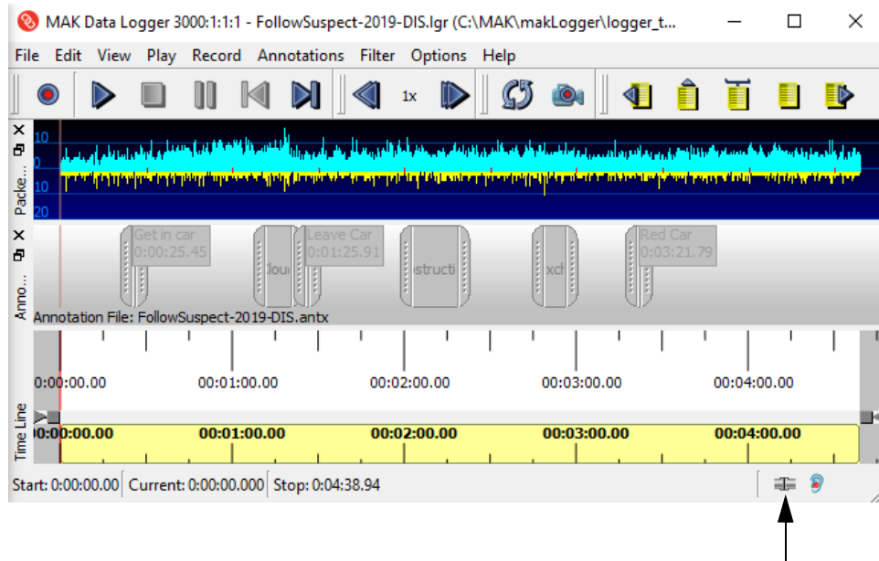
Figure 4-1. Connection status
