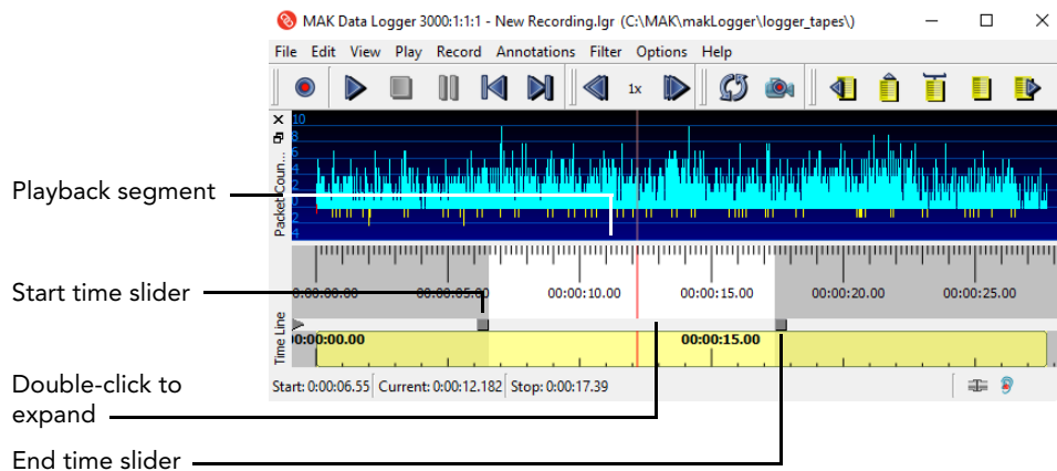
Figure 8-1. Timeline sliders
