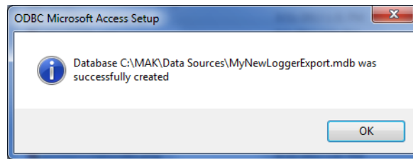
Figure 13-8. Information prompt
