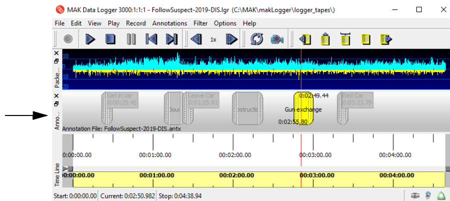
Figure 9-1. Annotations display
