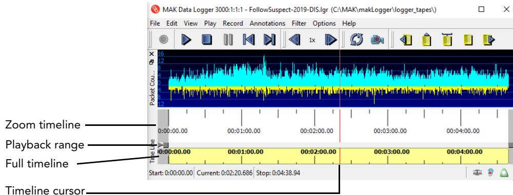
Figure 6-2. Timeline
