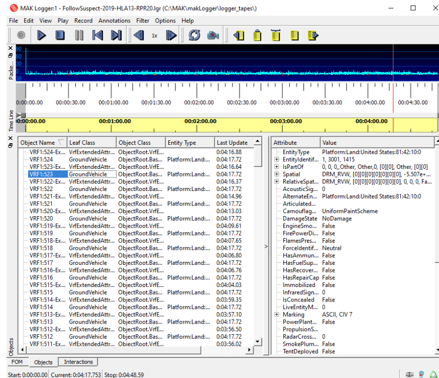
Figure 11-2. Objects tab
