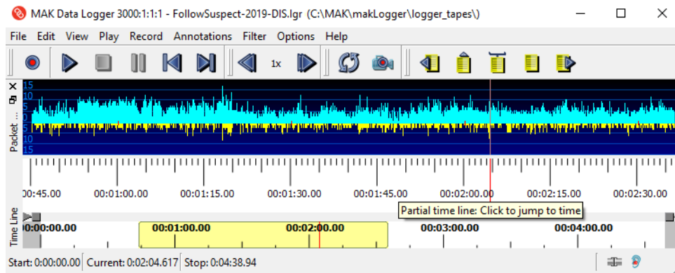
Figure 8-4. Zoomed timeline
