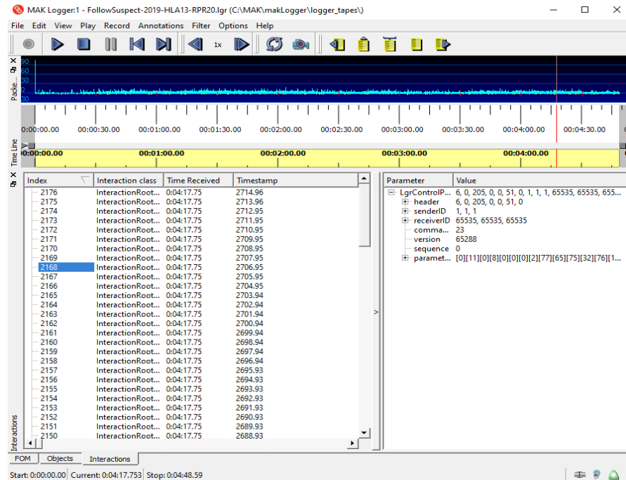
Figure 11-3. Interactions tab
