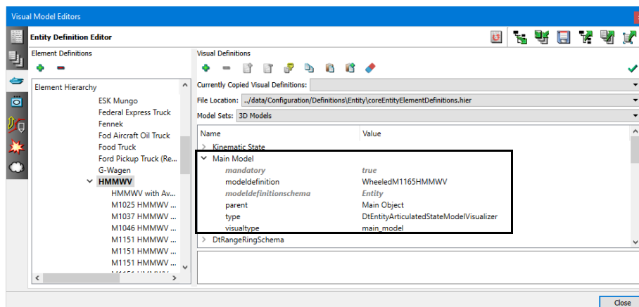
Figure 12-2. Model definition for Main Model
