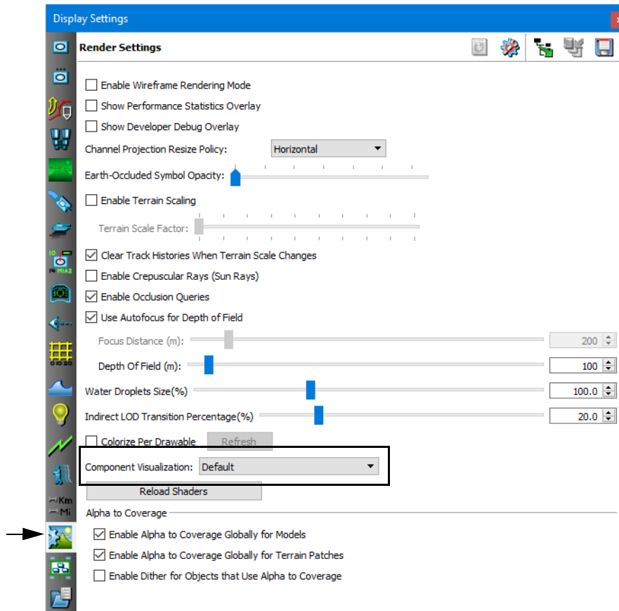
Figure 10-5. Render Settings page
