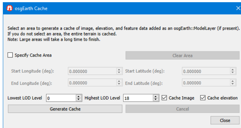
Figure 10-2. osgEarth Cache dialog box
