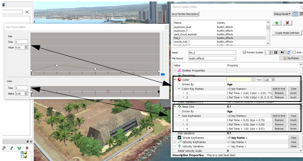
Figure 20-2. Key Frame Editor and keyframe properties
