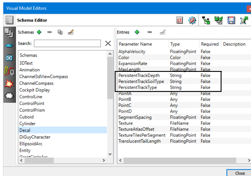
Figure 17-15. Persistent track parameters in Decal Schema
