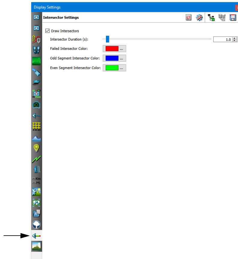
Figure 10-6. Intersector Settings page
