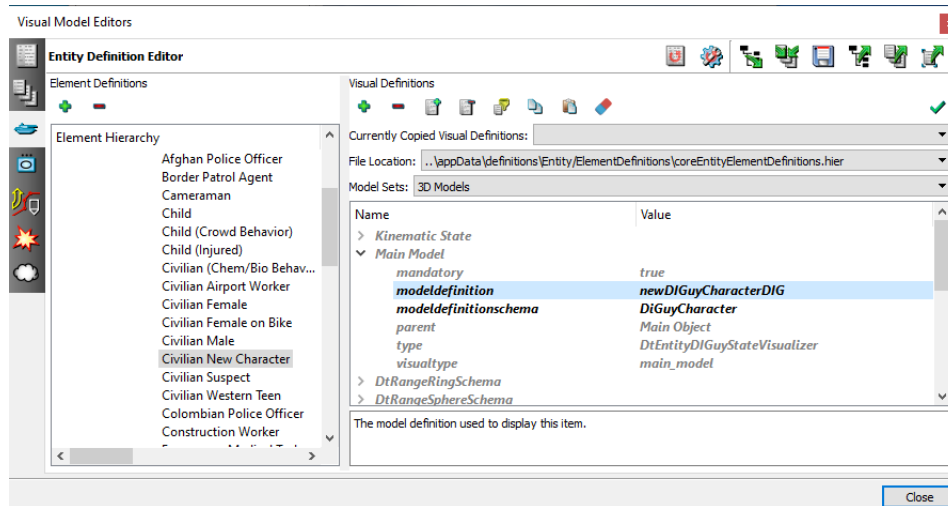
Figure 23-10. Completed entity definition
