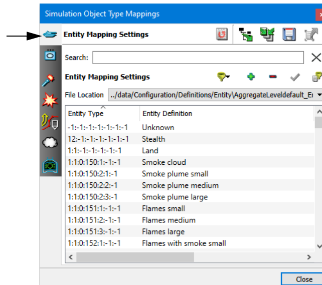
Figure 16-1. Entity Mapping Settings page
