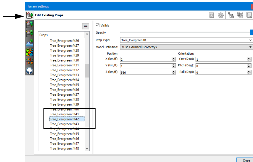
Figure 11-7. Edit Existing Props page
