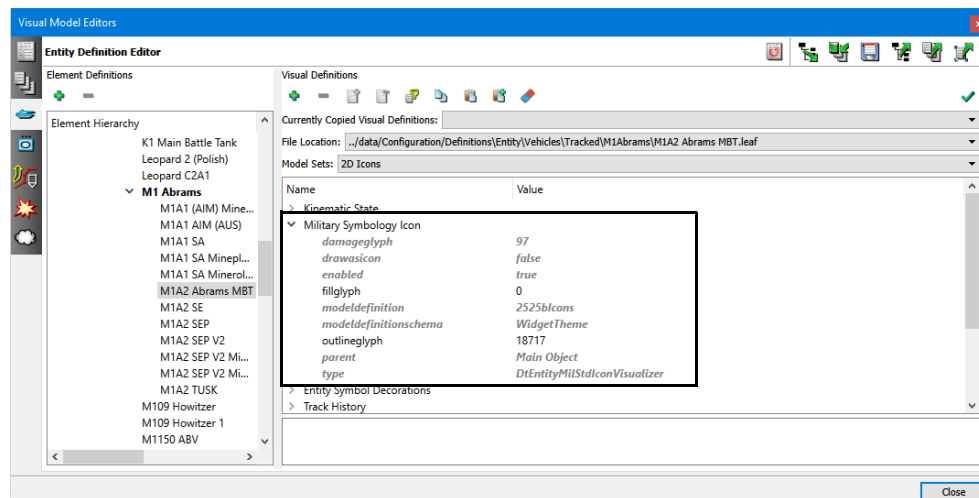
Figure 17-1. Military Symbol Icon visual definition
