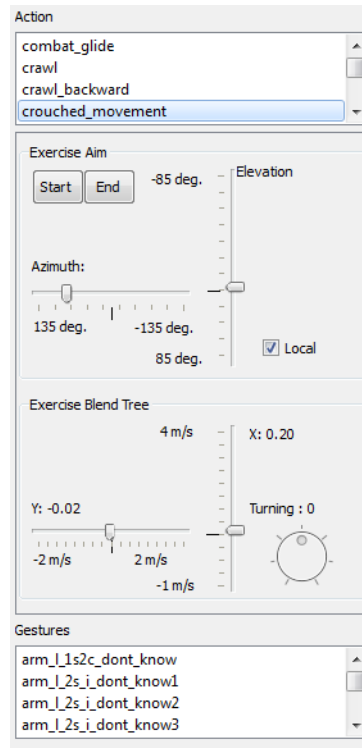
Figure 22-3. Exercise Aim panel
