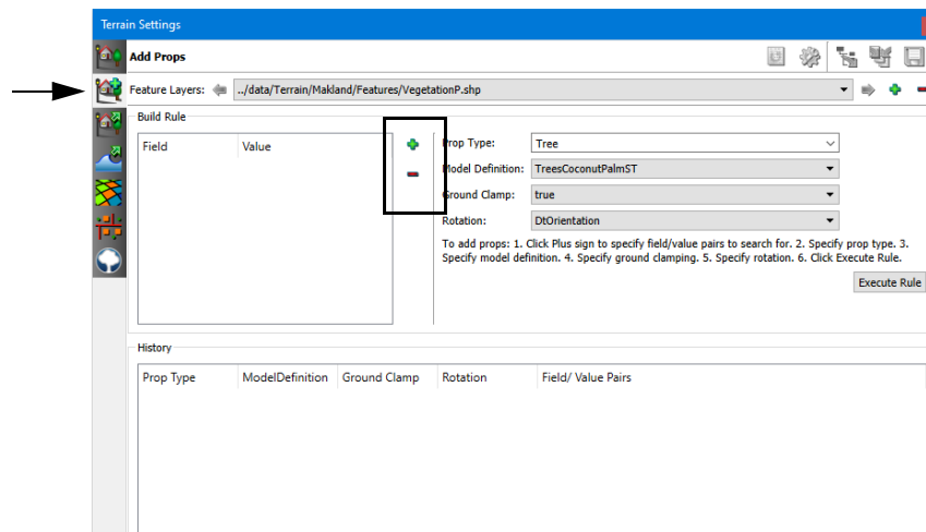
Figure 1-12. Terrain Settings, Add Props page
