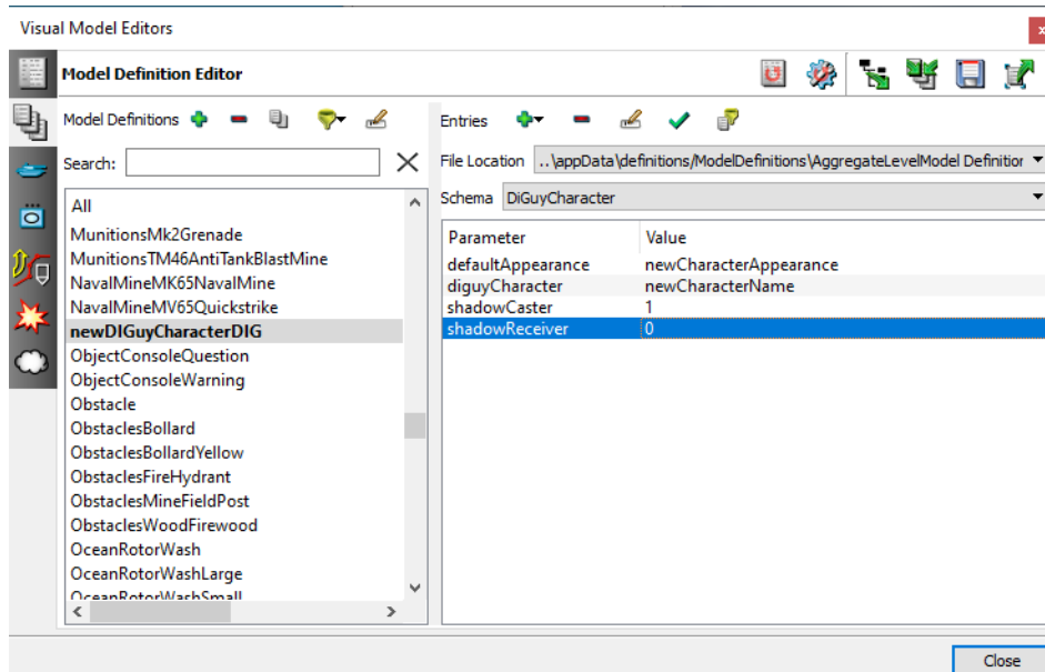
Figure 23-4. DI-Guy character parameters
