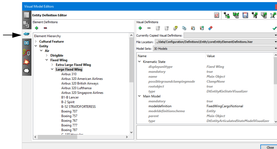
Figure 15-1. Entity Definition Editor page
