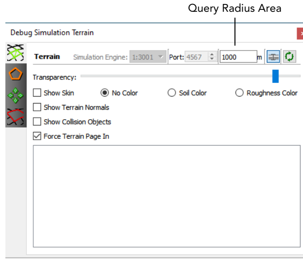
Figure 10-10. Simulation Terrain Debugging Tool
