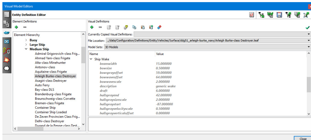
Figure 17-14. Ship Wake visual definition
