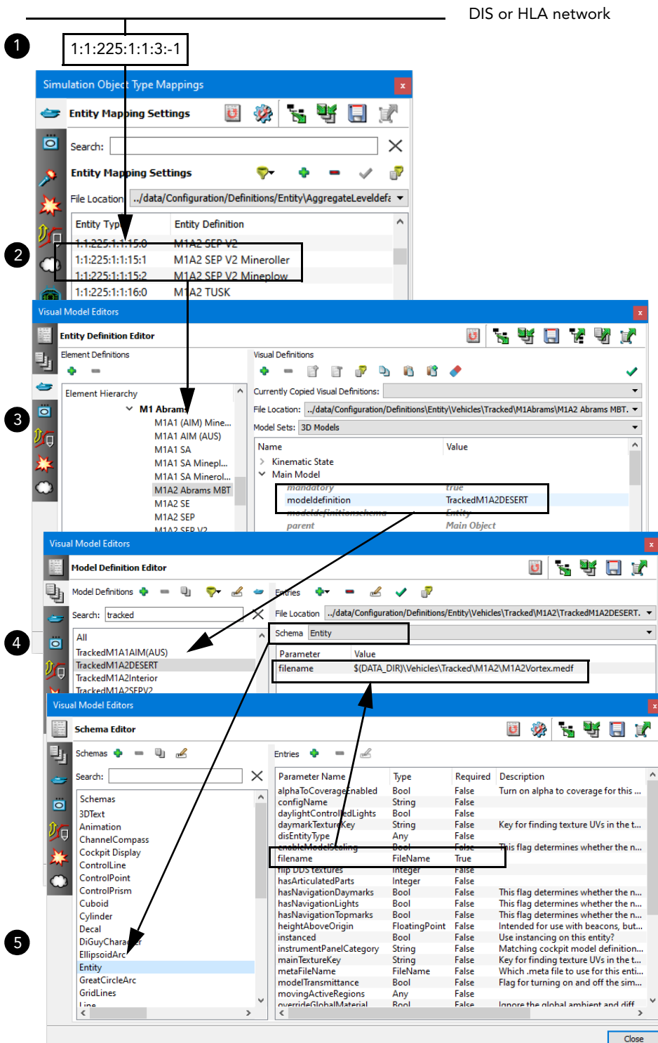
Figure 12-1. Element definitions and simulation object type mapping
