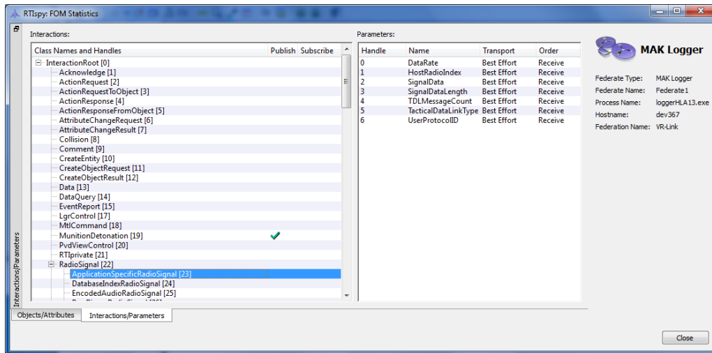
Figure 7-2. RTIsPy: Federate FOM, interaction classes
