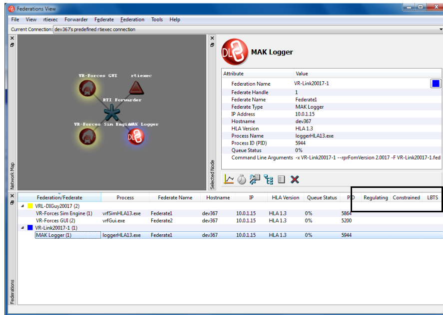
Figure 6-2. Time management state information
