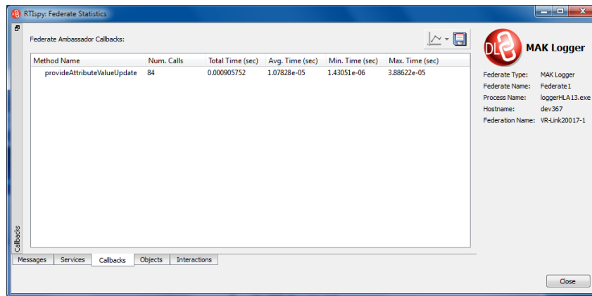
Figure 8-11. RTIspy Federate Statistics, Callbacks tab
