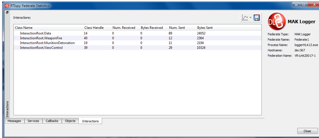
Figure 8-8. RTIsPy Federate Statistics, Interactions tab
