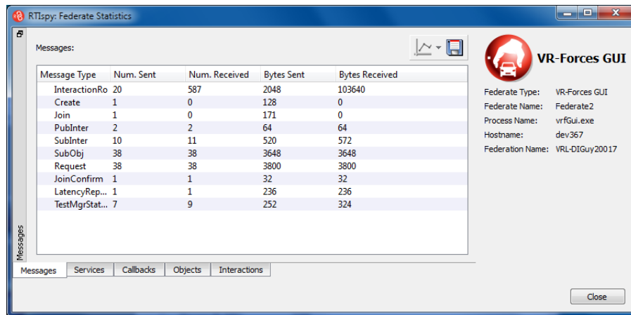
Figure 8-9. RTISpy Federate Statistics, Messages tab
