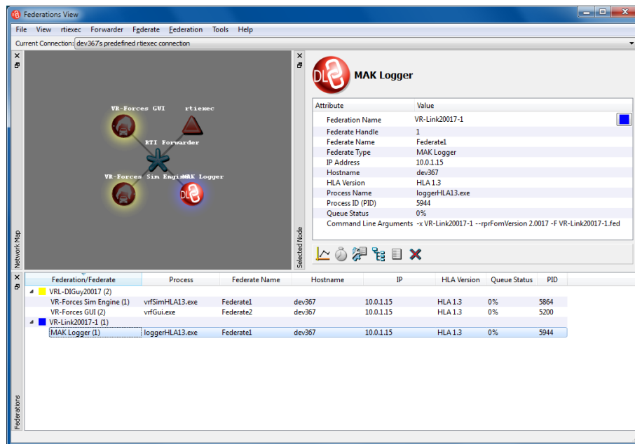
Figure 4-1. Federations View
