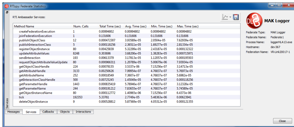
Figure 8-10. RTISpy Federate Statistics, Services tab
