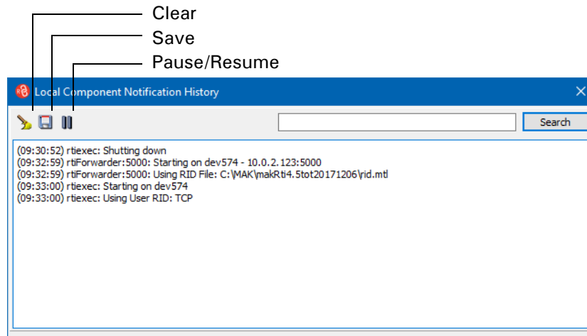
Figure 5-3. Console window
