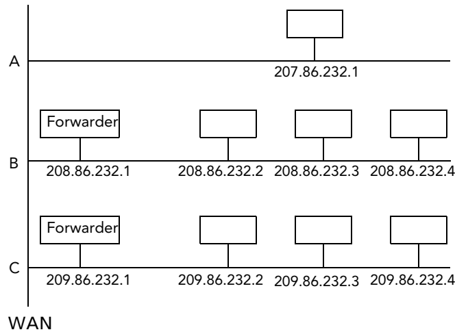
Figure 10-7. UDP forwarding
