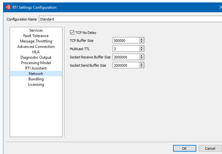
Figure 9-5. Network page
