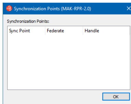
Figure 6-3. Synchronization points
