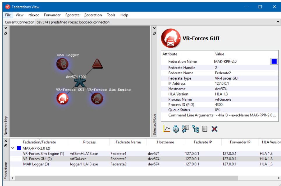
Figure 5-4. Federations View
