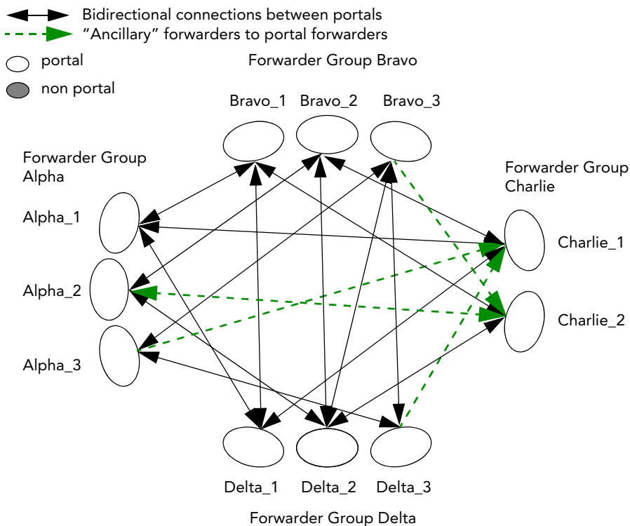
Figure 10-5. Distributed Forwarder Network (load-balanced)
