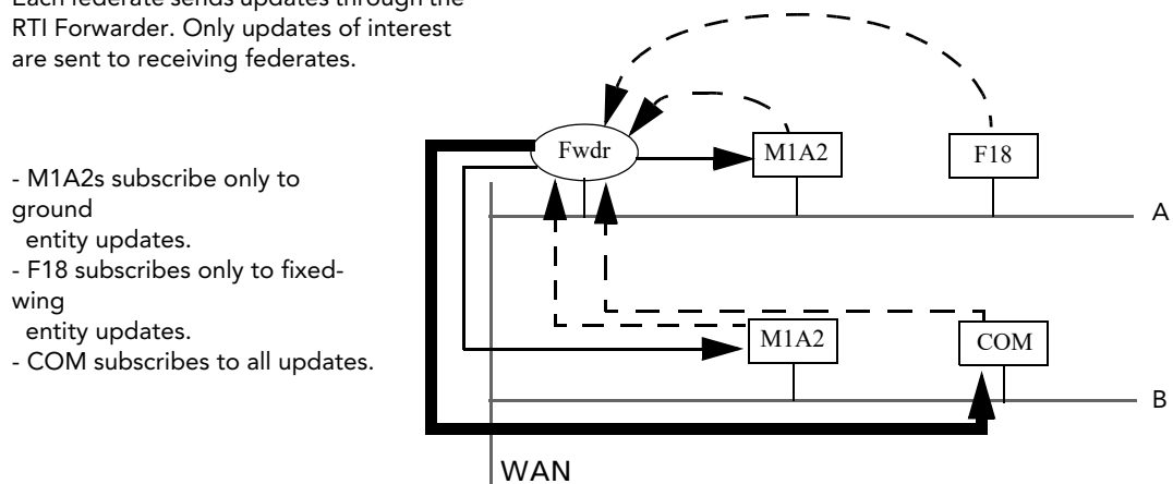
Figure 9-3. TCP forwarding compared to sender-side filtering
