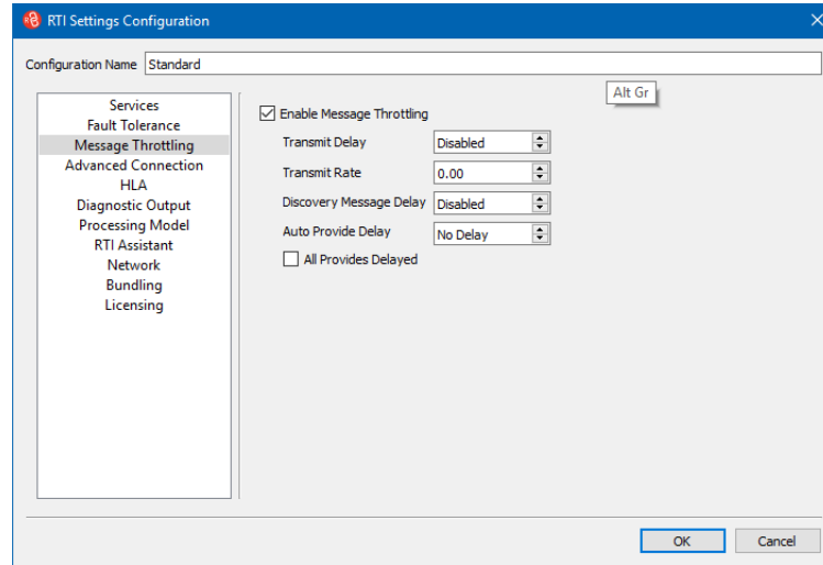
Figure 9-7. Message Throttling page
