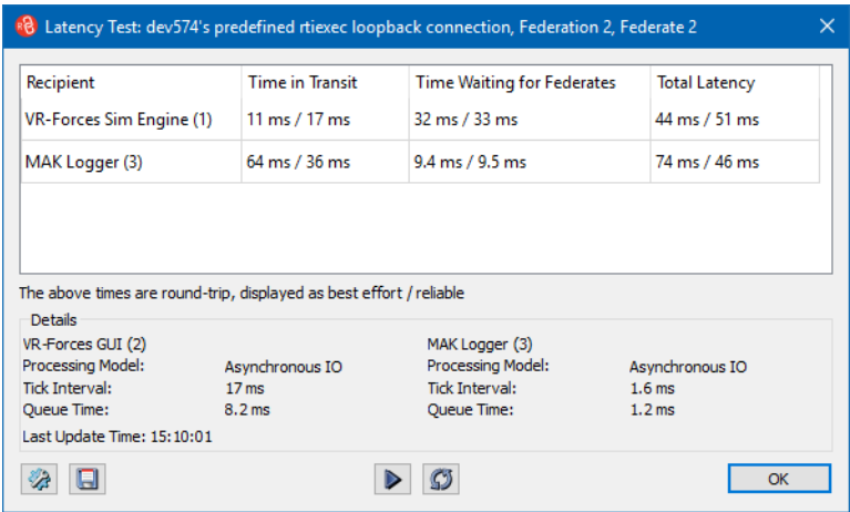
Figure 8-1. Latency Test window
