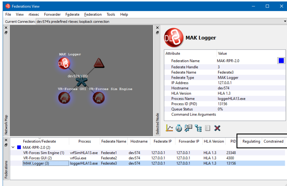
Figure 6-2. Time management state information
