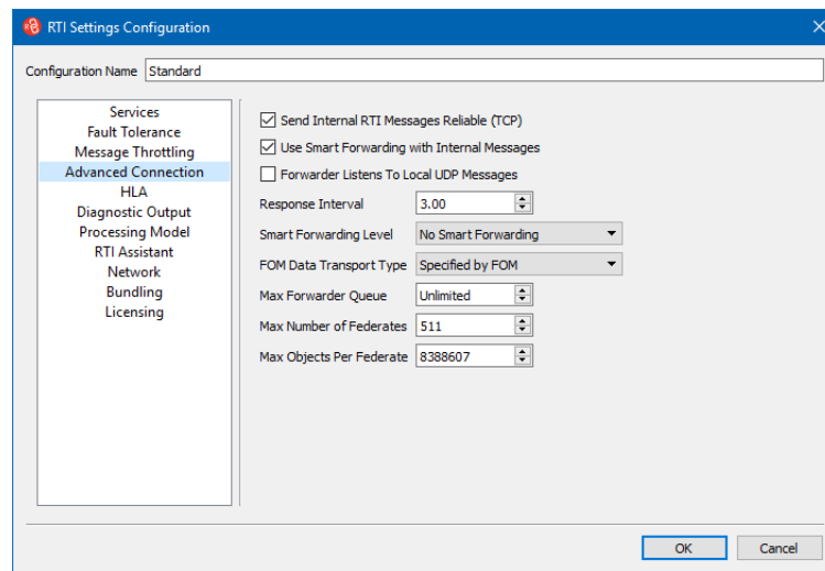
Figure 9-4. Advanced Connection page
