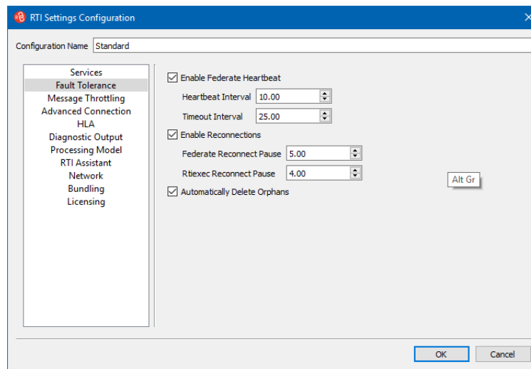
Figure 6-7. Fault Tolerance page
