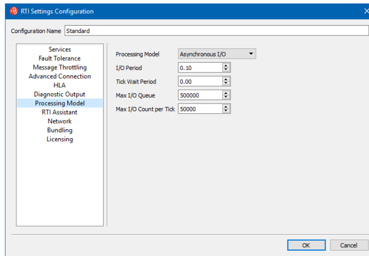
Figure 9-6. Processing Model page
