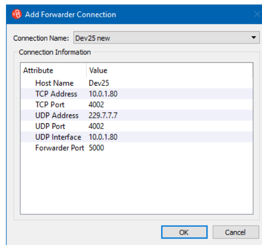
Figure 10-8. Add Forwarder Connection dialog box
