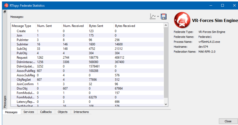
Figure 8-10. RTIspy Federate Statistics, Messages tab
