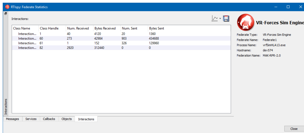
Figure 8-9. RTIspy Federate Statistics, Interactions tab
