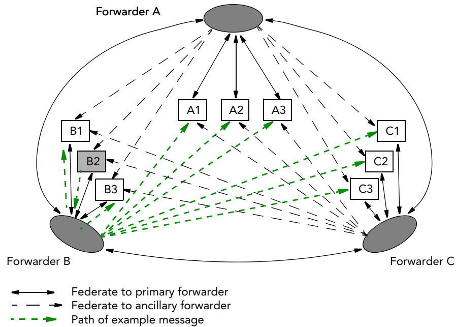
Figure 10-1. Distributed forwarding on a LAN with a forwarder group
