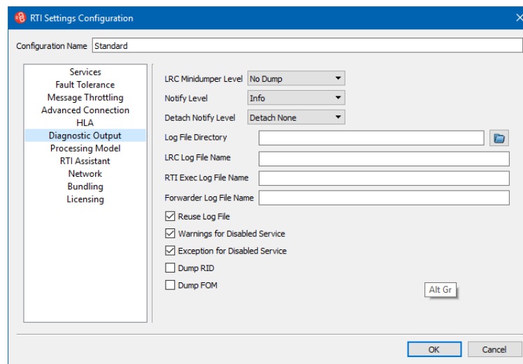
Figure 6-9. Diagnostic Output page
