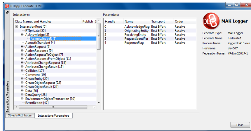
Figure 7-2. RTIsPy: Federate FOM, interaction classes
