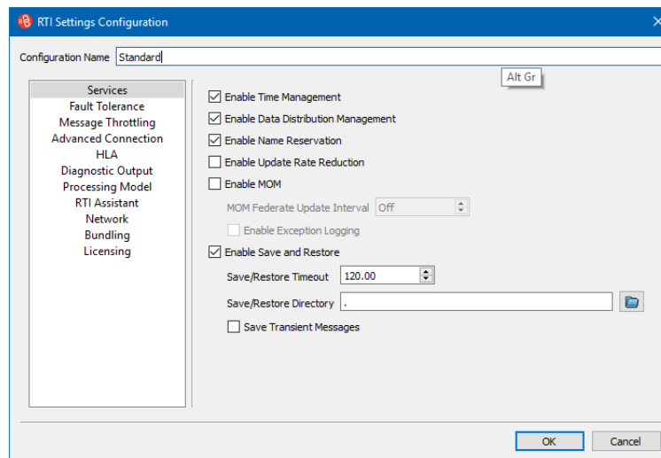
Figure 4-2. RTI Settings Configuration dialog box
