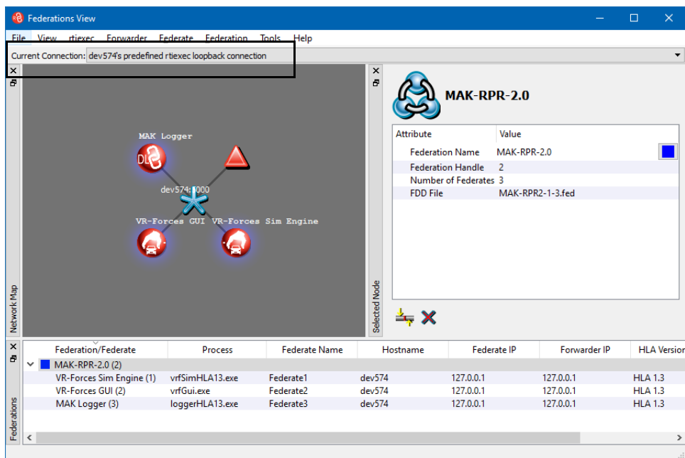
Figure 6-1. RTI Federation View, federation selected
