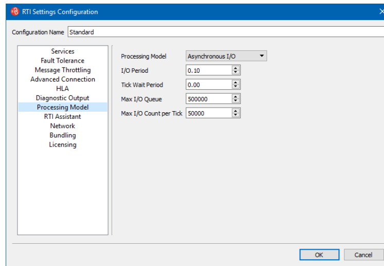
Figure 6-8. Processing Model page
