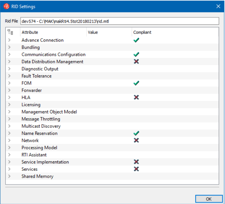
Figure 4-4. RID Settings dialog box
