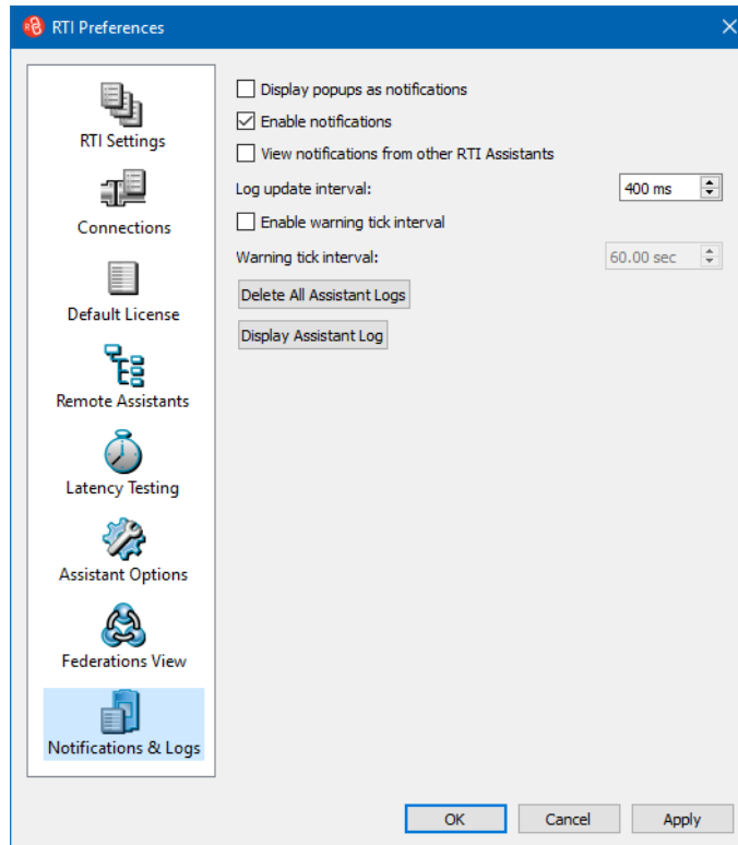
Figure 5-1. RTI Preferences dialog box, Notifications and Logs
