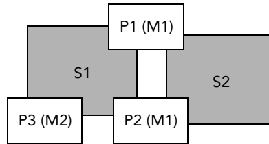
Figure 12-3. Distributed region using subscription regions
