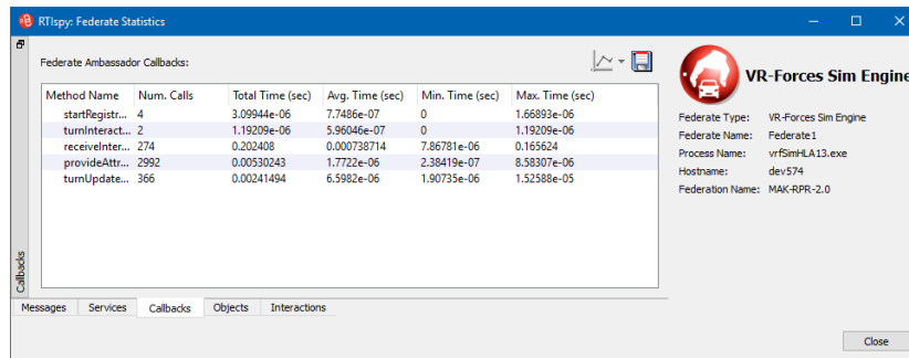
Figure 8-12. RTIsPy Federate Statistics, Callbacks tab
