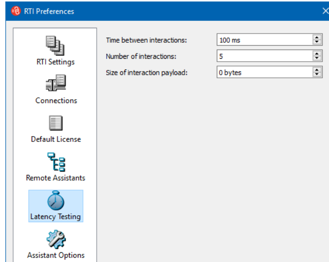
Figure 8-5. RTI Preferences dialog box, Latency Testing page
