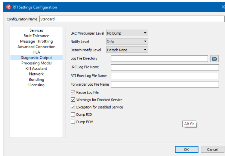
Figure 7-3. Diagnostic Output page
