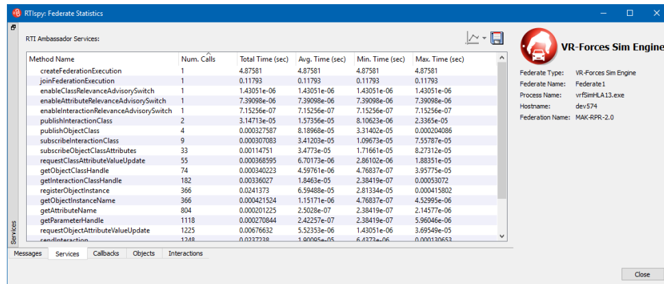
Figure 8-11. RTIsPy Federate Statistics, Services tab
