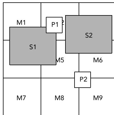
Figure 12-4. Fixed grid approach with overlaid regions
