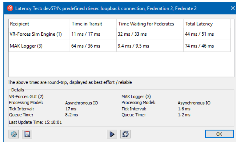
Figure 8-2. Latency test results, best effort only
