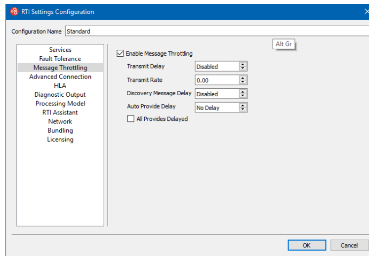
Figure 11-3. Message Throttling page
