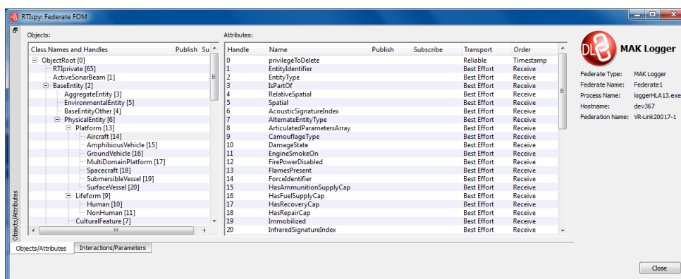
Figure 7-1. RTIsPy: Federate FOM, object classes
