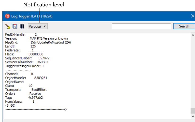
Figure 7-4. Federate Log window
