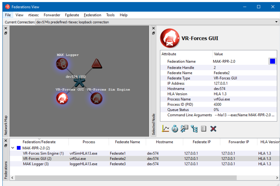
Figure 5-1. Federations View
