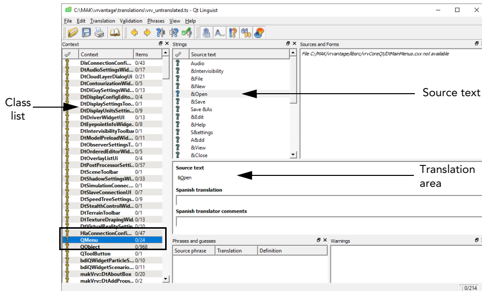
Figure 2-5. Linguist window
