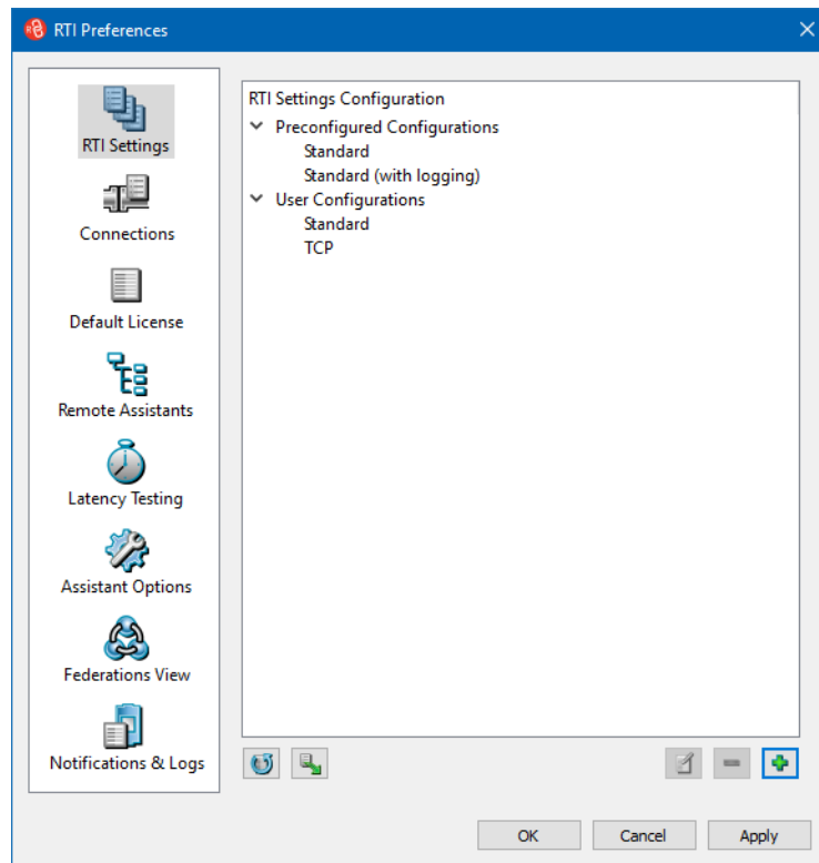
Figure 2-1. RTI Preferences
