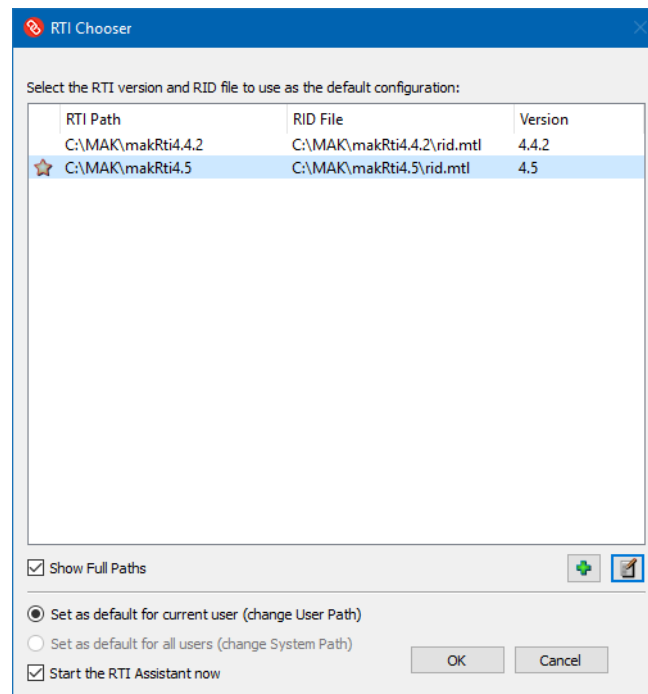
Figure 7-1. RTI Chooser
