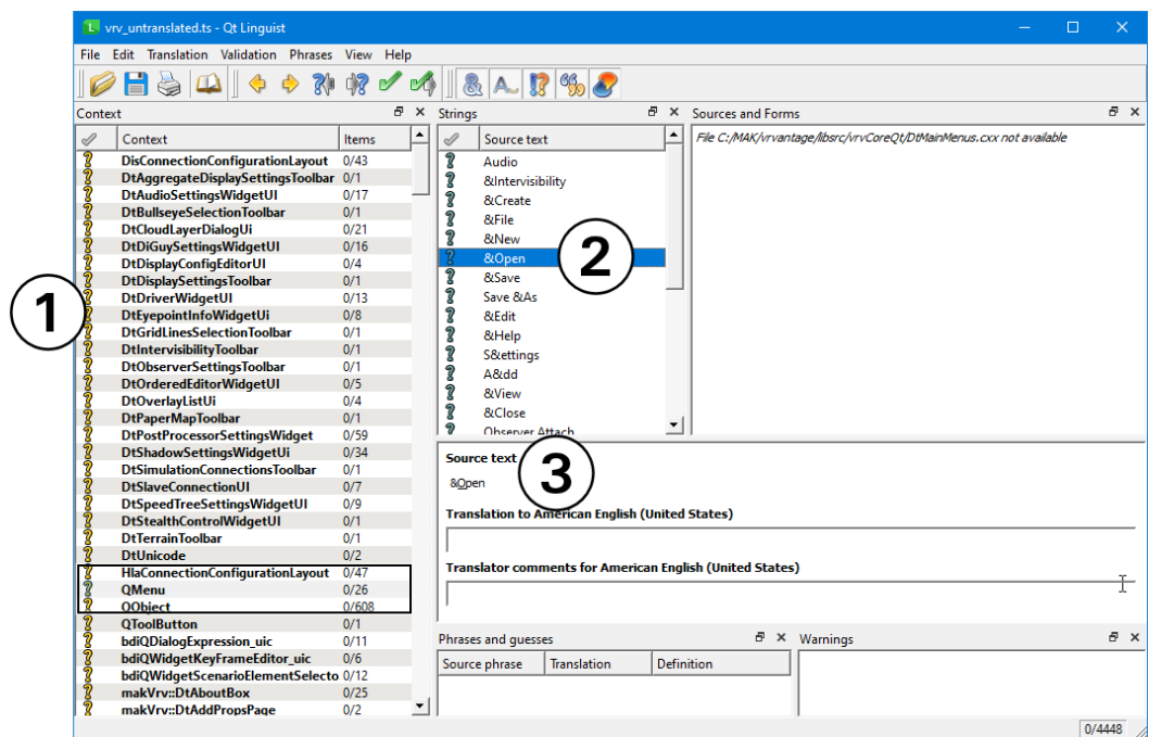
Figure 6. Linguist window
