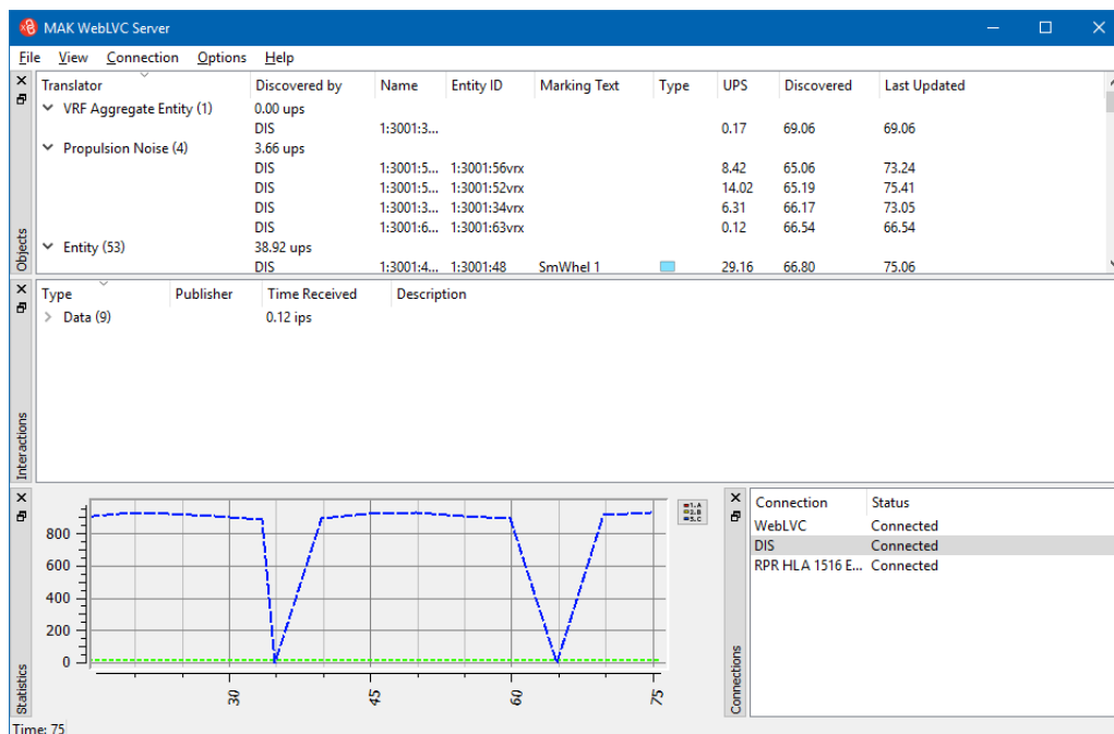
Figure 3-1. WebLVC Server Portal
