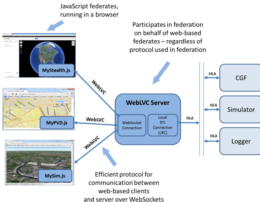
Figure 1-1. WebLVC protocol
