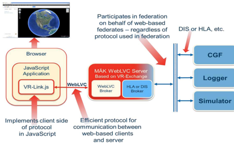
Figure 1-1. WebLVC Server
