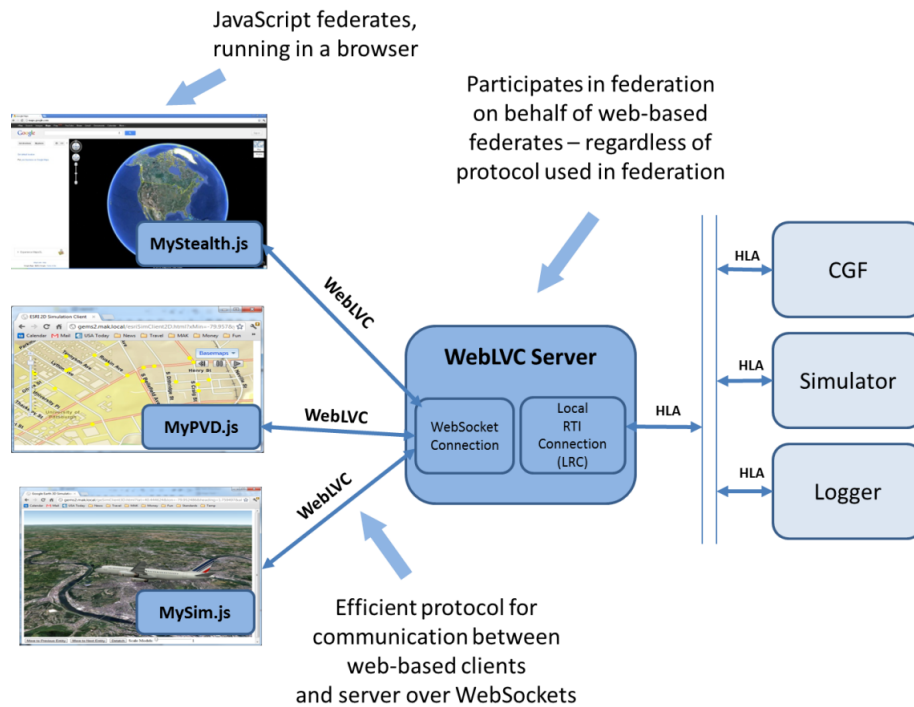
Figure 1-1. WebLVC protocol
