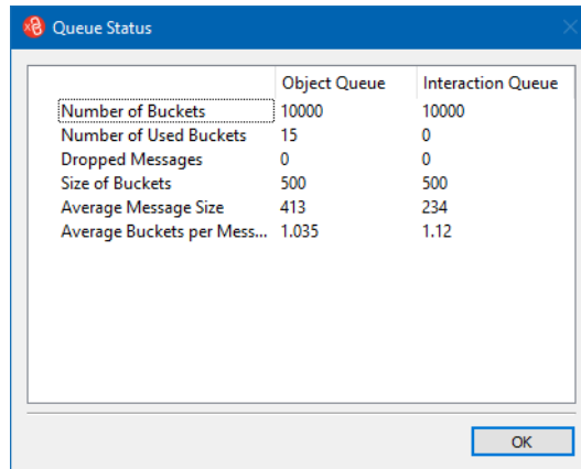
Figure 5-8. Queue Status dialog box
