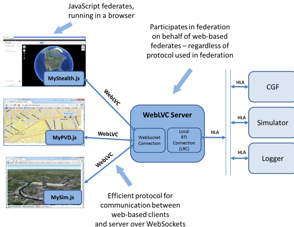
Figure 1. WebLVC protocol
