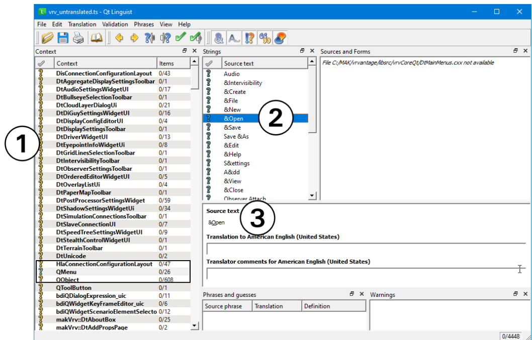
Figure 6. Linguist window
