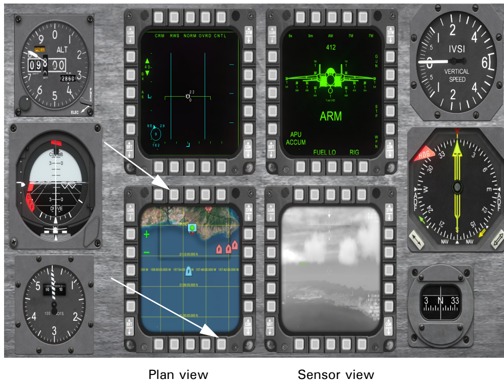
Figure 1-22. Multi-function displays
