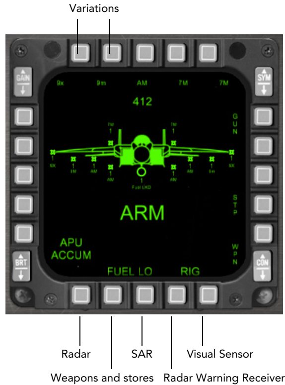
Figure 2-24. Multi-function display
