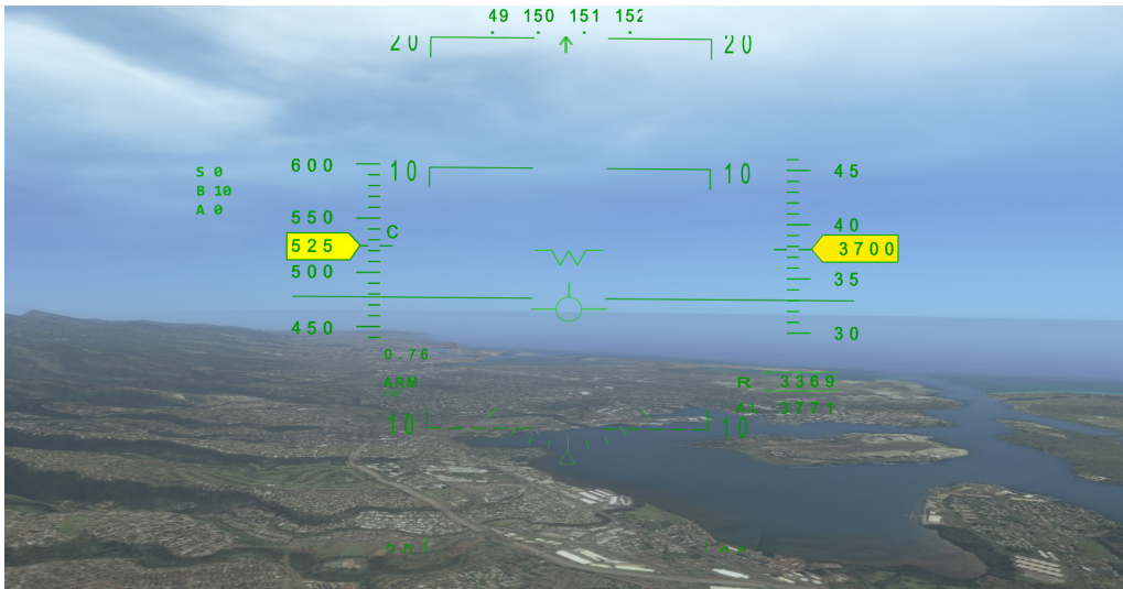
Figure 2-23. HUD (2 Screen display)
